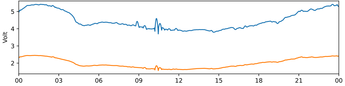
Tjautjas 30 MHz and 38 MHz riometer 2024-05-27 UTC
