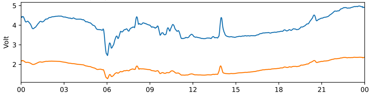
Tjautjas 30 MHz and 38 MHz riometer 2024-05-17 UTC
