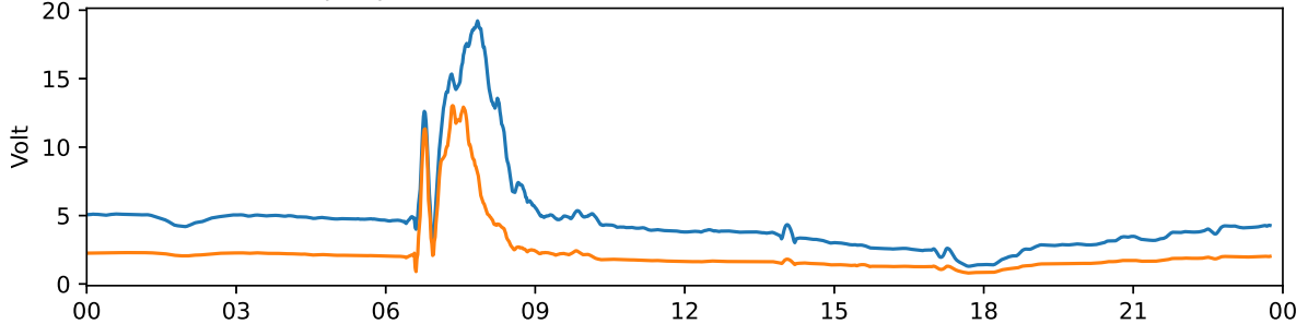
Tjautjas 30 MHz and 38 MHz riometer 2024-05-11 UTC
