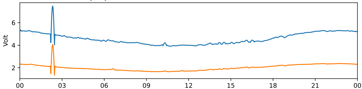
Tjautjas 30 MHz and 38 MHz riometer 2024-06-27 UTC
