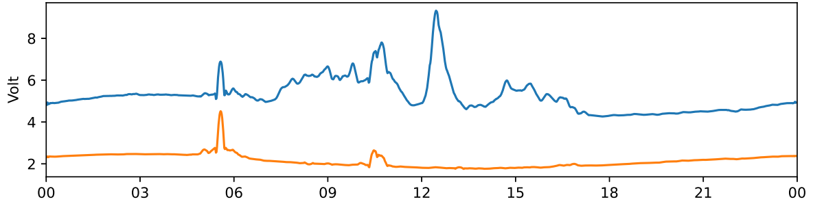
Tjautjas 30 MHz and 38 MHz riometer 2024-04-15 UTC
