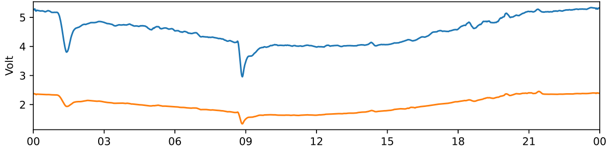
Tjautjas 30 MHz and 38 MHz riometer 2024-06-02 UTC
