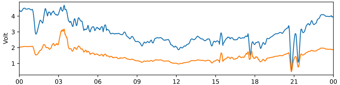
Tjautjas 30 MHz and 38 MHz riometer 2024-05-12 UTC
