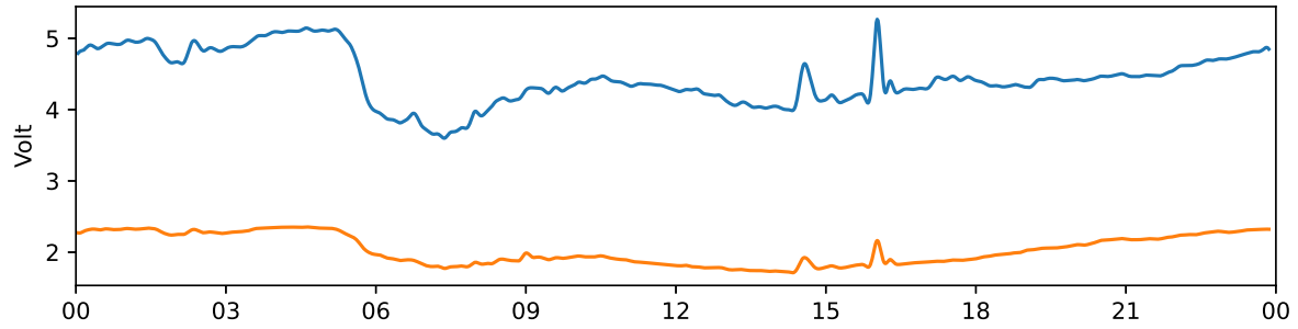
Tjautjas 30 MHz and 38 MHz riometer 2024-04-09 UTC
