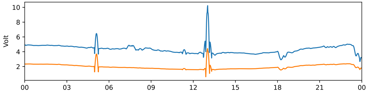
Tjautjas 30 MHz and 38 MHz riometer 2024-05-18 UTC
