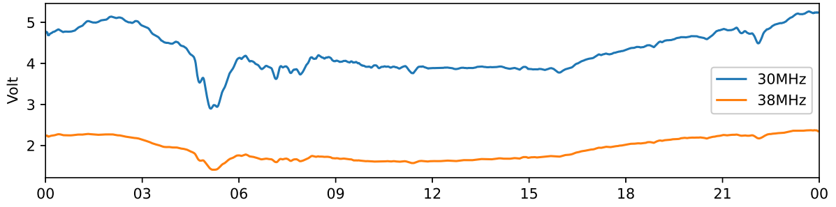
Tjautjas 30 MHz and 38 MHz riometer 2024-06-01 UTC
