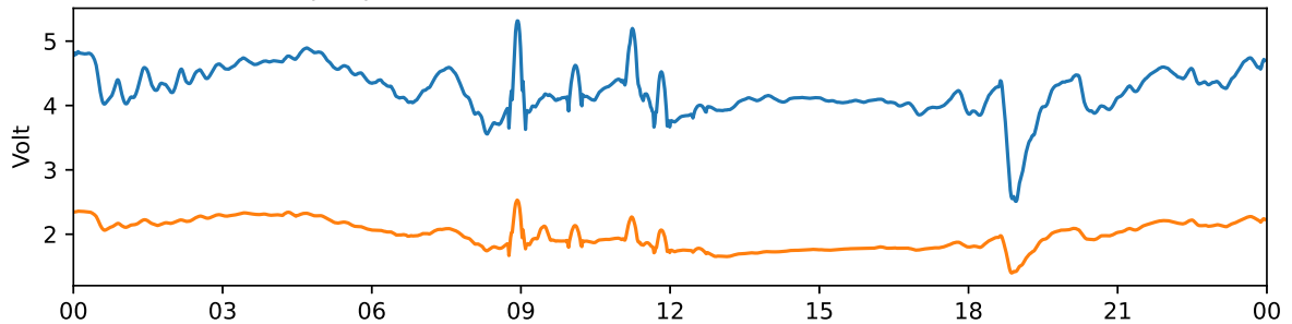
Tjautjas 30 MHz and 38 MHz riometer 2024-04-17 UTC
