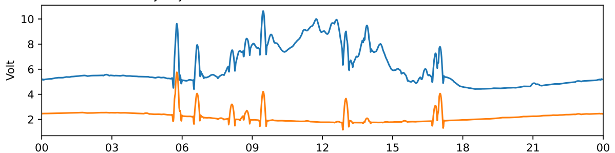
Tjautjas 30 MHz and 38 MHz riometer 2024-04-18 UTC
