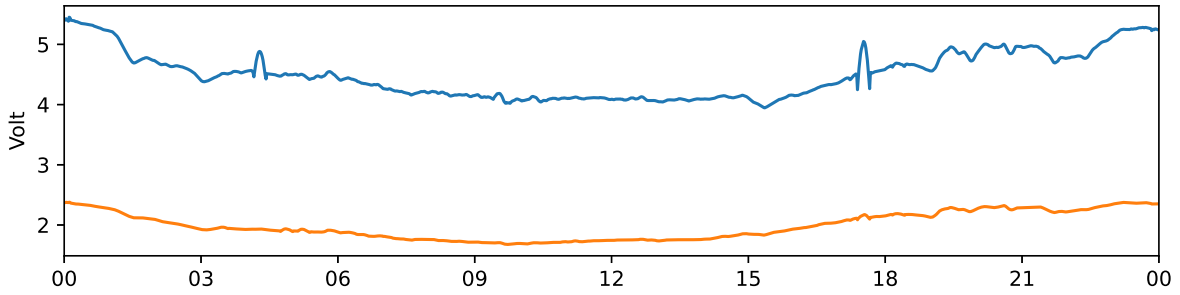
Tjautjas 30 MHz and 38 MHz riometer 2024-06-21 UTC
