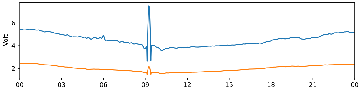
Tjautjas 30 MHz and 38 MHz riometer 2024-06-05 UTC
