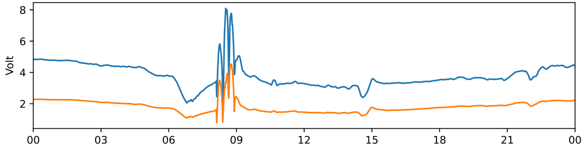
Tjautjas 30 MHz and 38 MHz riometer 2024-05-16 UTC
