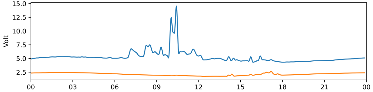
Tjautjas 30 MHz and 38 MHz riometer 2024-04-24 UTC
