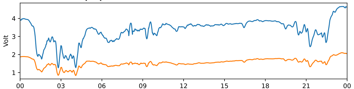
Tjautjas 30 MHz and 38 MHz riometer 2024-05-12 UTC
