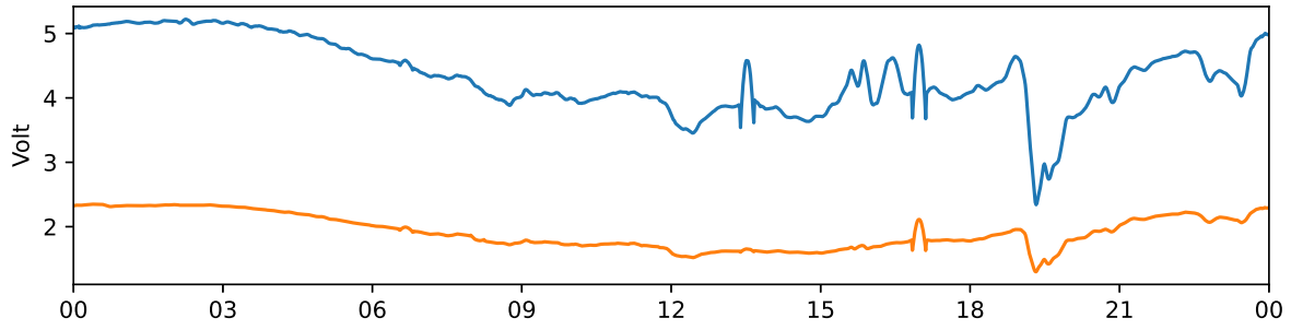
Tjautjas 30 MHz and 38 MHz riometer 2024-05-03 UTC
