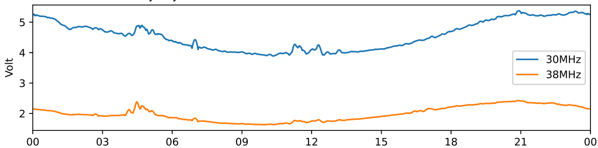
Tjautjas 30 MHz and 38 MHz riometer 2024-06-25 UTC
