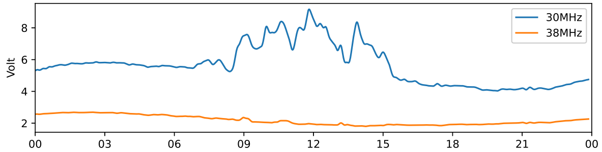
Tjautjas 30 MHz and 38 MHz riometer 2024-04-08 UTC
