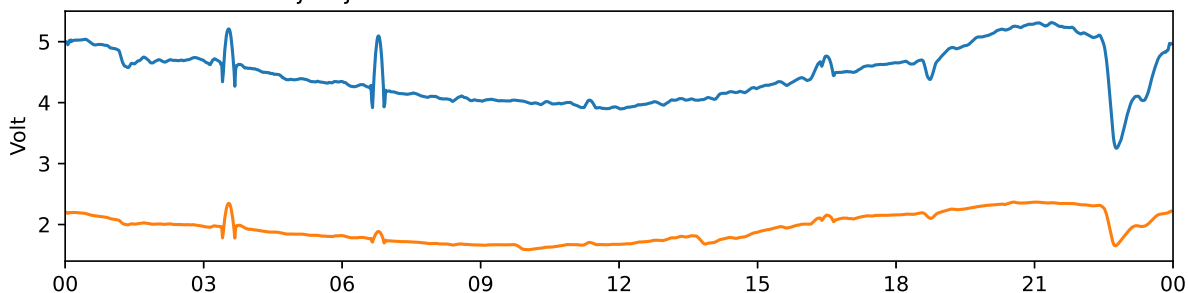
Tjautjas 30 MHz and 38 MHz riometer 2024-06-29 UTC
