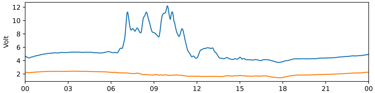
Tjautjas 30 MHz and 38 MHz riometer 2024-04-11 UTC
