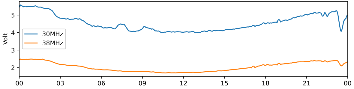
Tjautjas 30 MHz and 38 MHz riometer 2024-05-26 UTC
