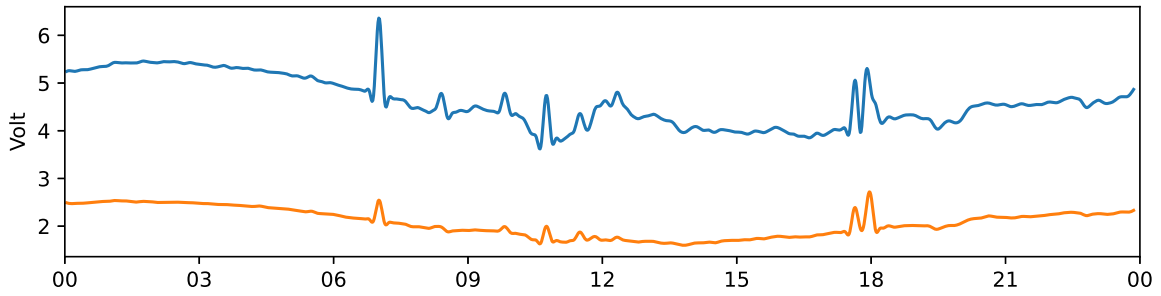
Tjautjas 30 MHz and 38 MHz riometer 2024-04-24 UTC
