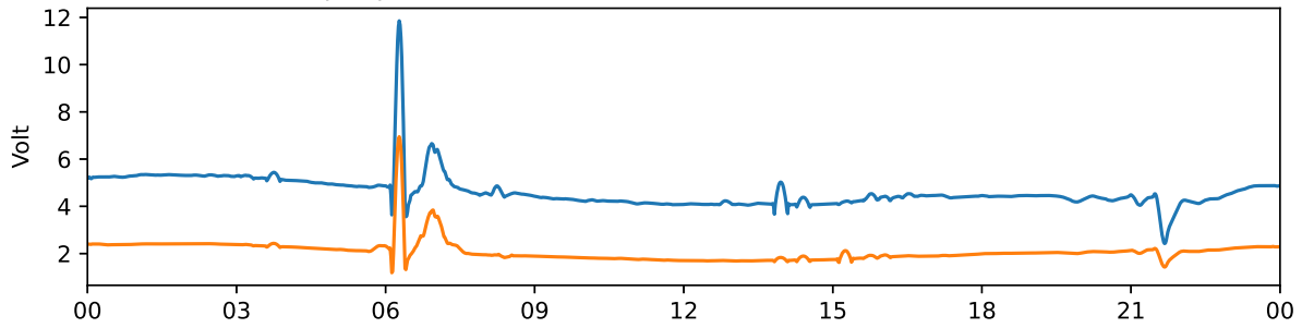
Tjautjas 30 MHz and 38 MHz riometer 2024-05-05 UTC
