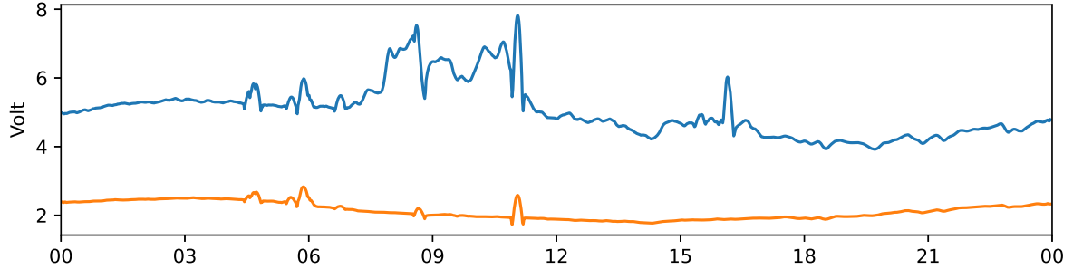
Tjautjas 30 MHz and 38 MHz riometer 2024-04-16 UTC
