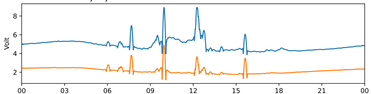
Tjautjas 30 MHz and 38 MHz riometer 2024-04-12 UTC
