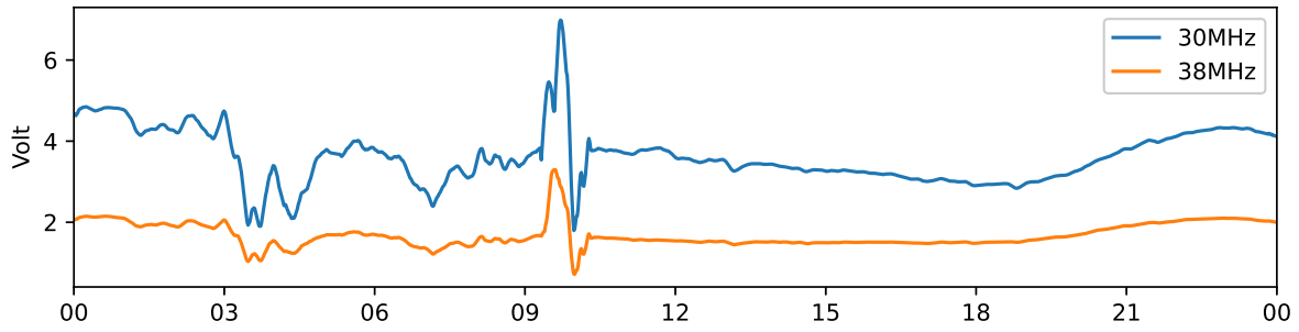
Tjautjas 30 MHz and 38 MHz riometer 2024-05-14 UTC
