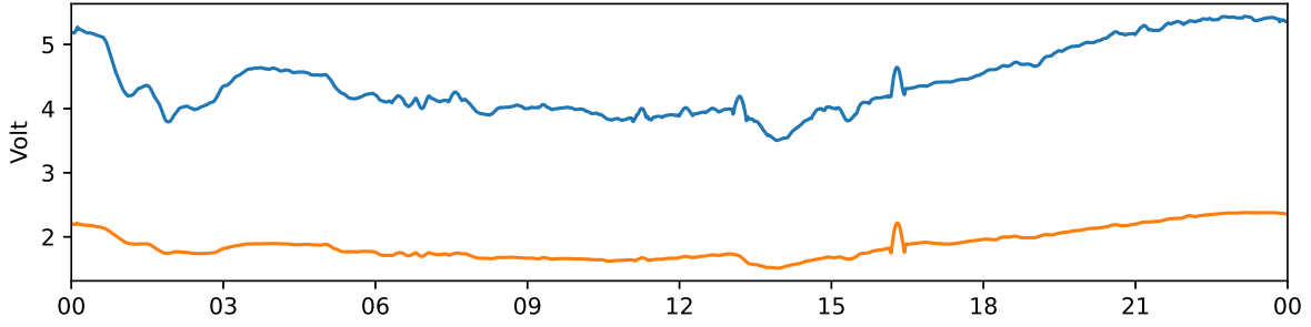
Tjautjas 30 MHz and 38 MHz riometer 2024-06-20 UTC
