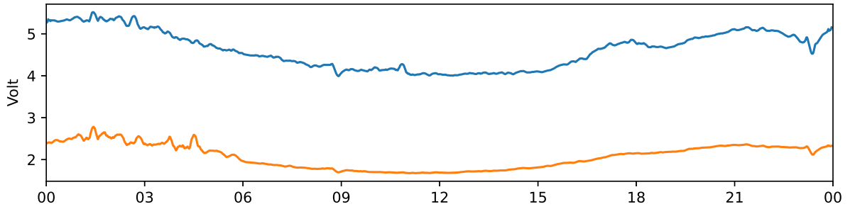
Tjautjas 30 MHz and 38 MHz riometer 2024-06-03 UTC
