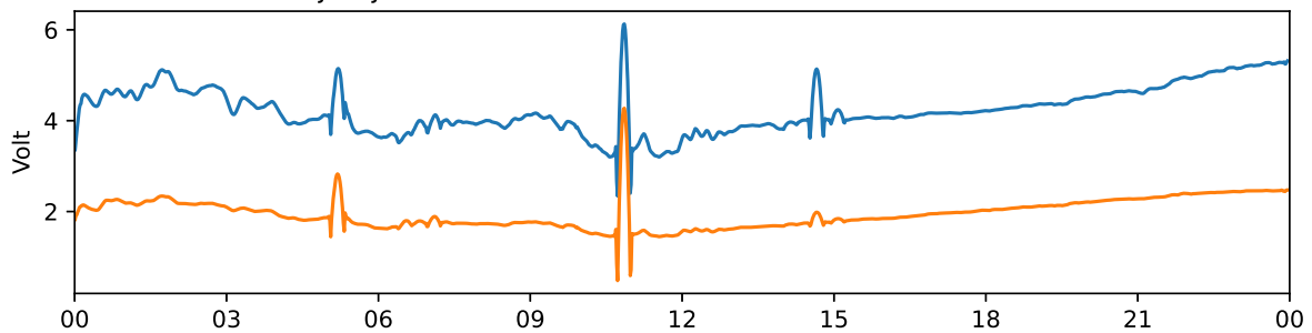
Tjautjas 30 MHz and 38 MHz riometer 2024-05-18 UTC
