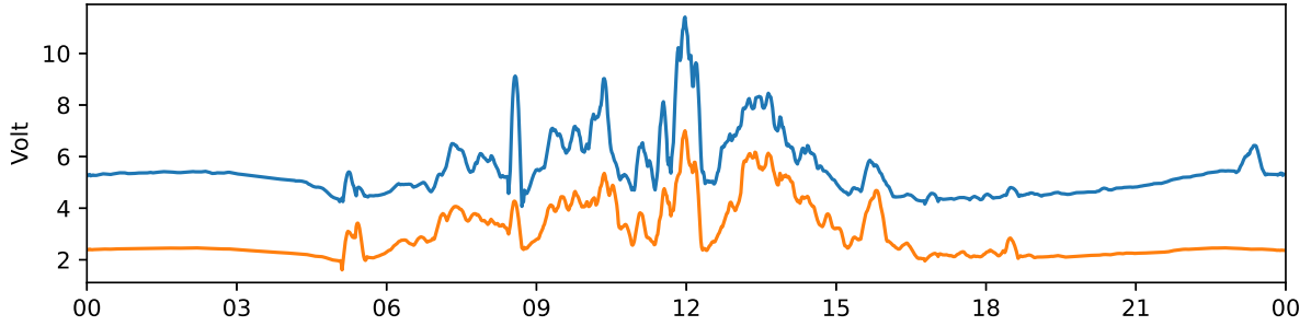
Tjautjas 30 MHz and 38 MHz riometer 2024-05-09 UTC
