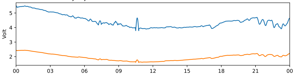
Tjautjas 30 MHz and 38 MHz riometer 2024-05-30 UTC
