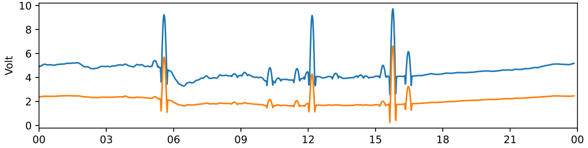
Tjautjas 30 MHz and 38 MHz riometer 2024-04-23 UTC
