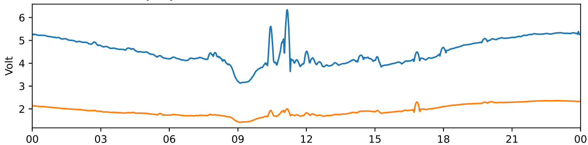
Tjautjas 30 MHz and 38 MHz riometer 2024-06-26 UTC
