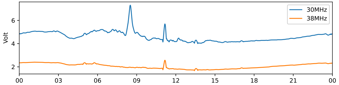
Tjautjas 30 MHz and 38 MHz riometer 2024-04-14 UTC
