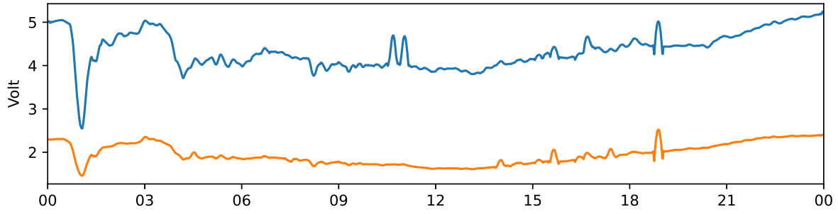
Tjautjas 30 MHz and 38 MHz riometer 2024-05-04 UTC
