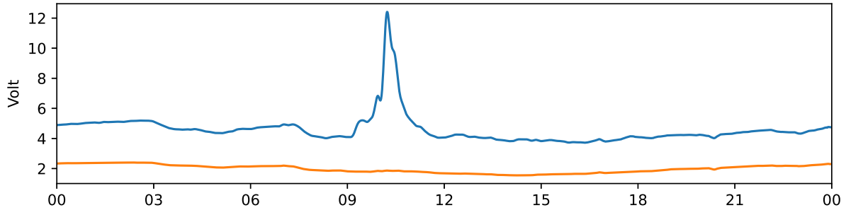
Tjautjas 30 MHz and 38 MHz riometer 2024-04-10 UTC
