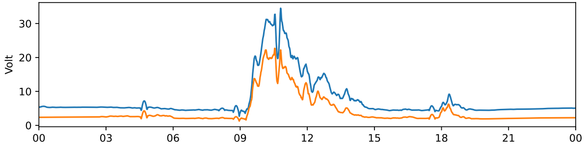
Tjautjas 30 MHz and 38 MHz riometer 2024-05-10 UTC
