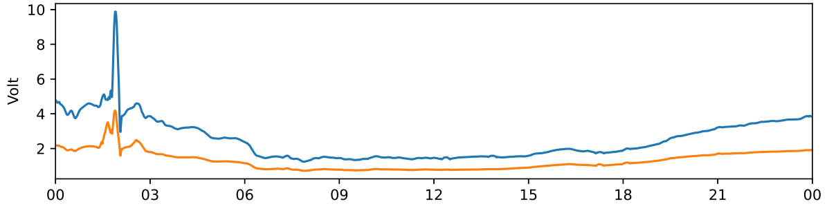
Tjautjas 30 MHz and 38 MHz riometer 2024-06-09 UTC
