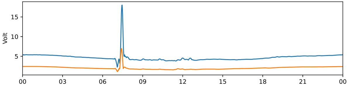
Tjautjas 30 MHz and 38 MHz riometer 2024-05-28 UTC
