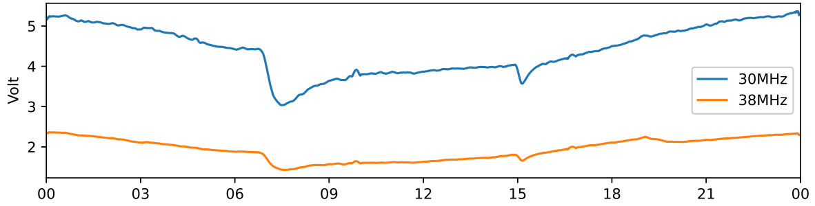
Tjautjas 30 MHz and 38 MHz riometer 2024-06-07 UTC
