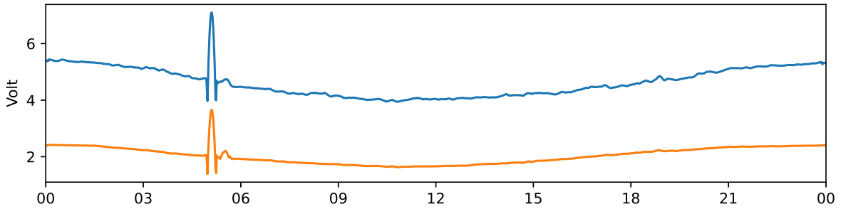
Tjautjas 30 MHz and 38 MHz riometer 2024-05-29 UTC
