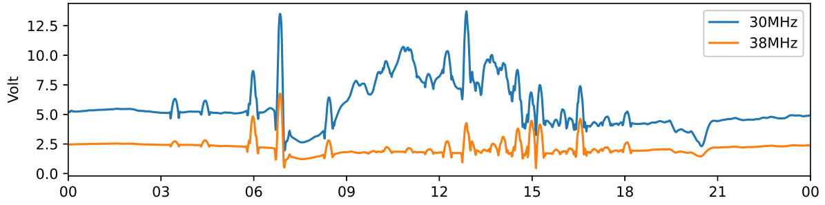
Tjautjas 30 MHz and 38 MHz riometer 2024-04-20 UTC
