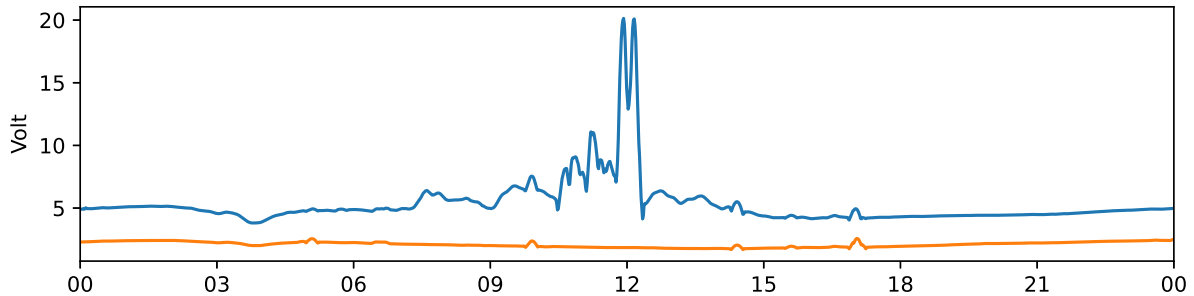
Tjautjas 30 MHz and 38 MHz riometer 2024-04-12 UTC
