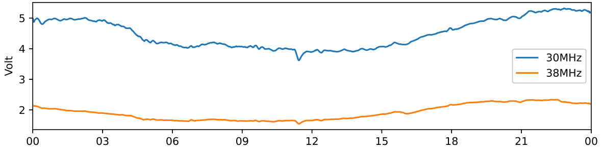
Tjautjas 30 MHz and 38 MHz riometer 2024-06-19 UTC
