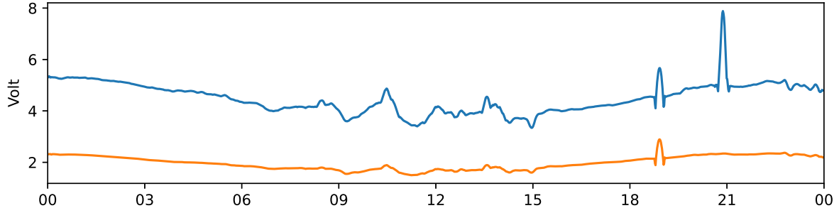
Tjautjas 30 MHz and 38 MHz riometer 2024-06-08 UTC
