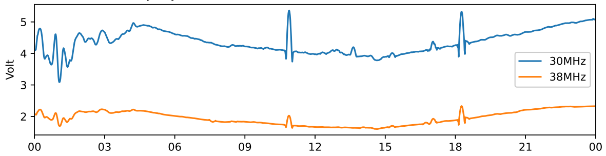
Tjautjas 30 MHz and 38 MHz riometer 2024-05-02 UTC
