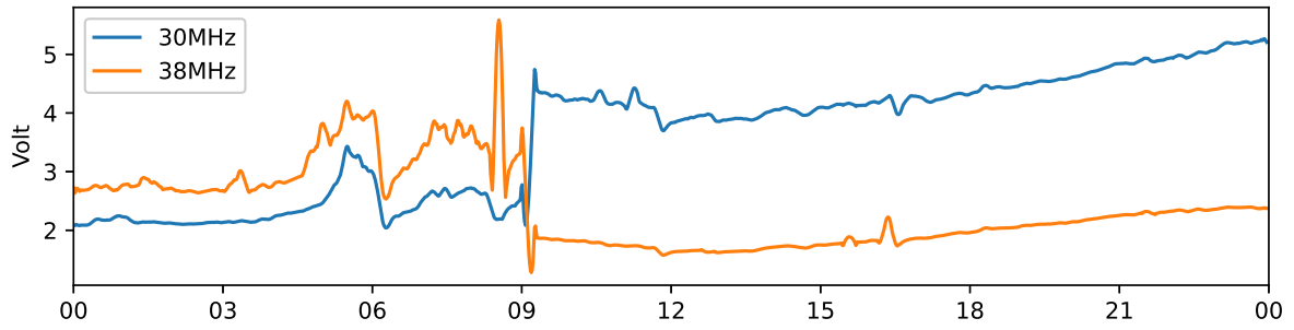
Tjautjas 30 MHz and 38 MHz riometer 2024-05-08 UTC
