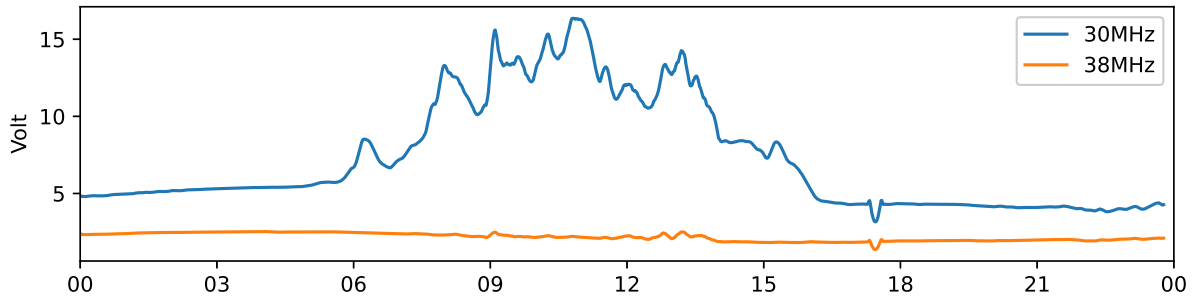
Tjautjas 30 MHz and 38 MHz riometer 2024-03-19 UTC
