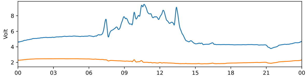
Tjautjas 30 MHz and 38 MHz riometer 2024-03-21 UTC
