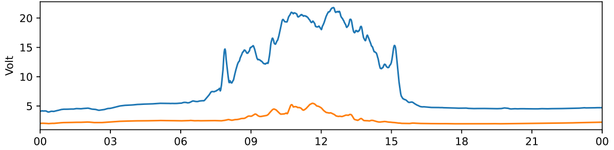
Tjautjas 30 MHz and 38 MHz riometer 2024-02-19 UTC
