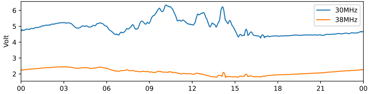
Tjautjas 30 MHz and 38 MHz riometer 2024-03-07 UTC
