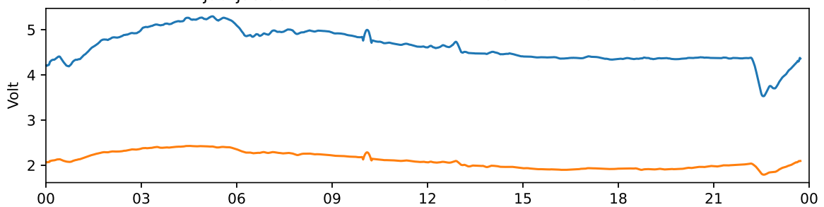
Tjautjas 30 MHz and 38 MHz riometer 2024-03-05 UTC
