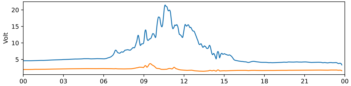
Tjautjas 30 MHz and 38 MHz riometer 2024-02-14 UTC
