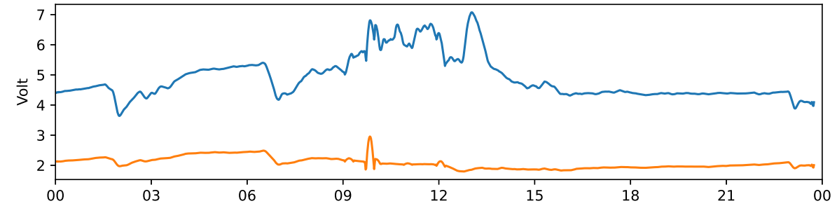
Tjautjas 30 MHz and 38 MHz riometer 2024-02-27 UTC
