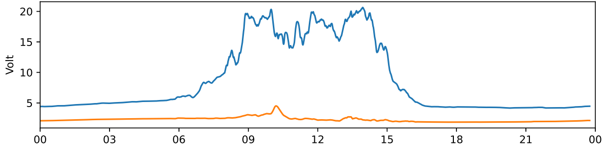
Tjautjas 30 MHz and 38 MHz riometer 2024-02-25 UTC
