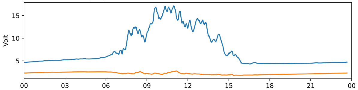
Tjautjas 30 MHz and 38 MHz riometer 2024-03-11 UTC
