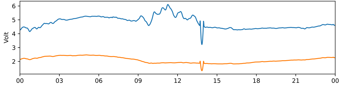
Tjautjas 30 MHz and 38 MHz riometer 2024-03-20 UTC
