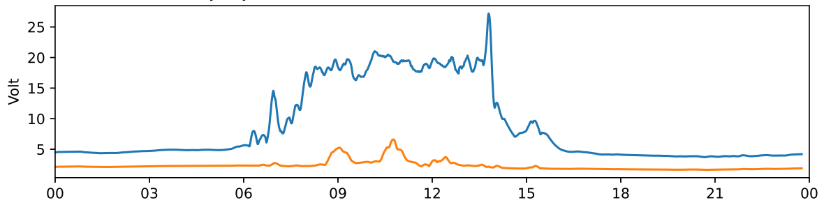
Tjautjas 30 MHz and 38 MHz riometer 2024-03-02 UTC
