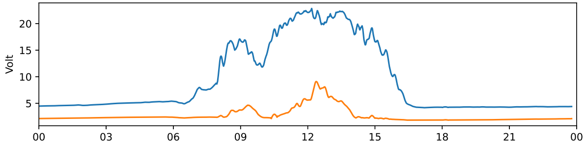
Tjautjas 30 MHz and 38 MHz riometer 2024-02-26 UTC
