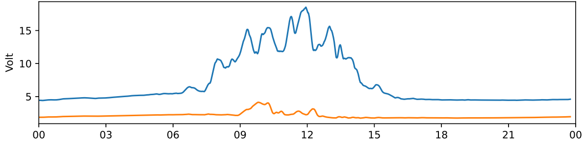
Tjautjas 30 MHz and 38 MHz riometer 2024-02-13 UTC
