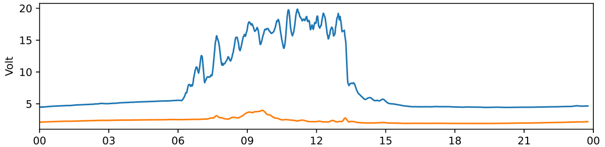
Tjautjas 30 MHz and 38 MHz riometer 2024-02-22 UTC
