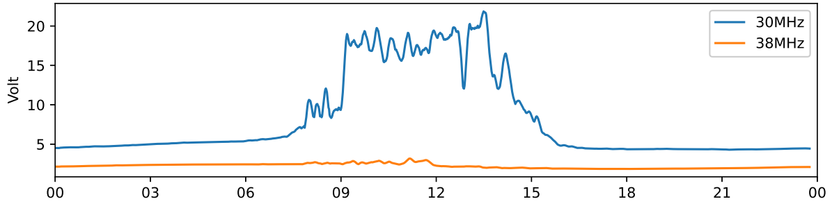
Tjautjas 30 MHz and 38 MHz riometer 2024-02-24 UTC
