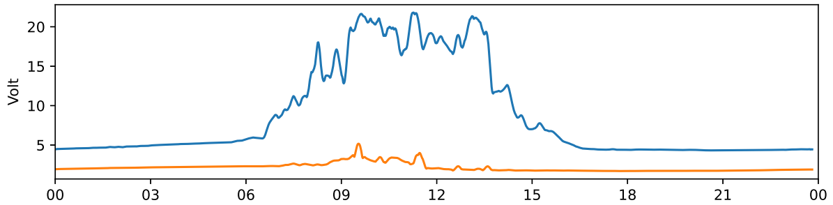
Tjautjas 30 MHz and 38 MHz riometer 2024-02-16 UTC
