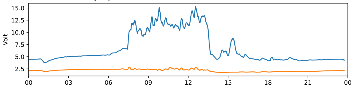
Tjautjas 30 MHz and 38 MHz riometer 2024-03-04 UTC
