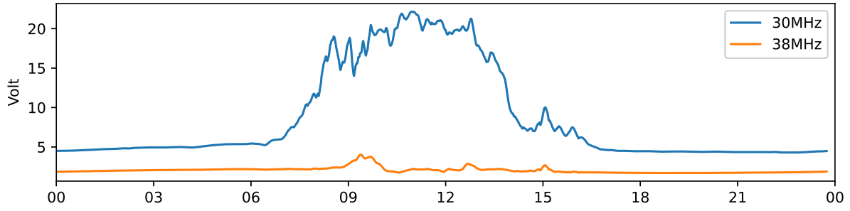
Tjautjas 30 MHz and 38 MHz riometer 2024-02-12 UTC
