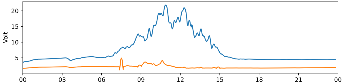
Tjautjas 30 MHz and 38 MHz riometer 2024-02-15 UTC
