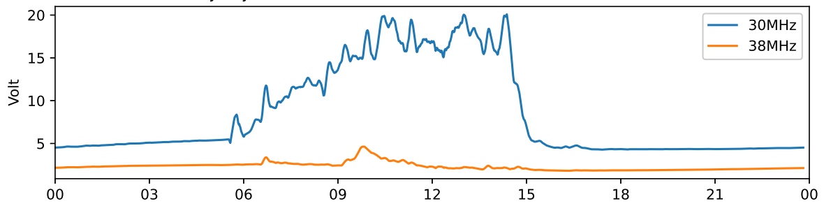
Tjautjas 30 MHz and 38 MHz riometer 2024-03-01 UTC
