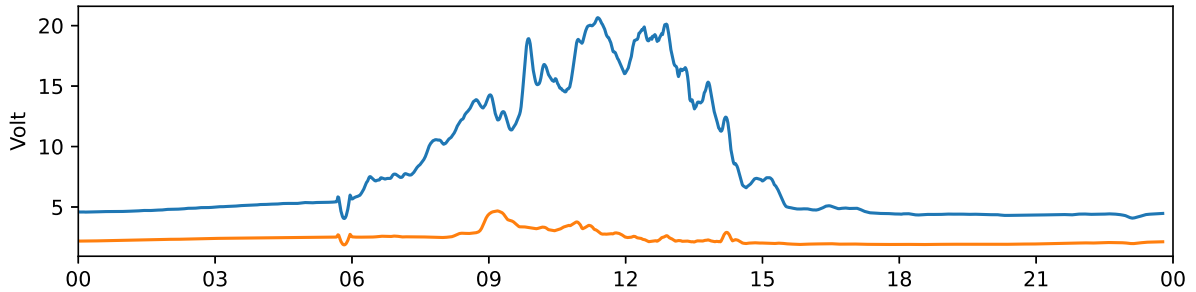
Tjautjas 30 MHz and 38 MHz riometer 2024-02-21 UTC
