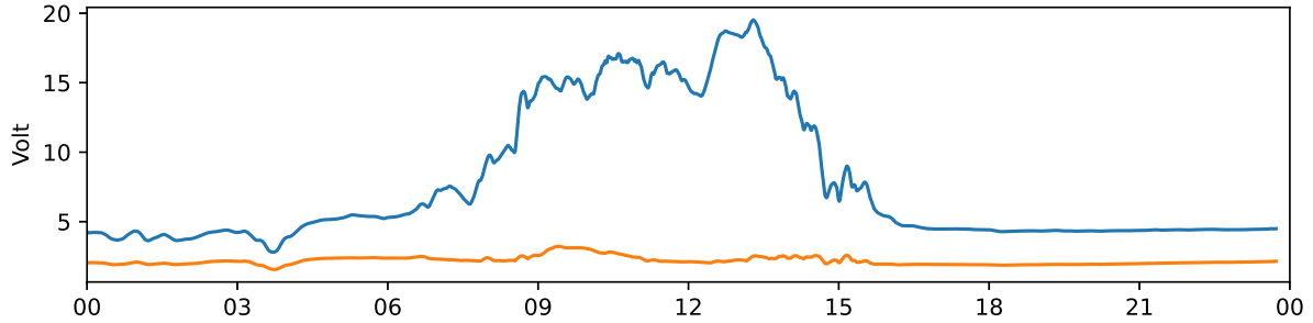
Tjautjas 30 MHz and 38 MHz riometer 2024-02-28 UTC
