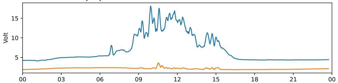
Tjautjas 30 MHz and 38 MHz riometer 2024-03-03 UTC
