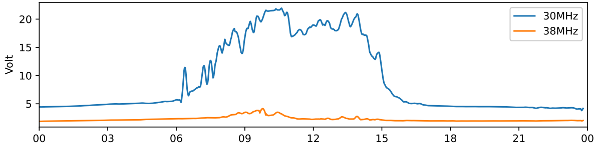
Tjautjas 30 MHz and 38 MHz riometer 2024-02-18 UTC
