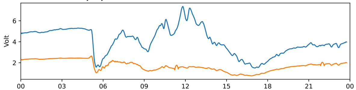
Tjautjas 30 MHz and 38 MHz riometer 2024-03-23 UTC
