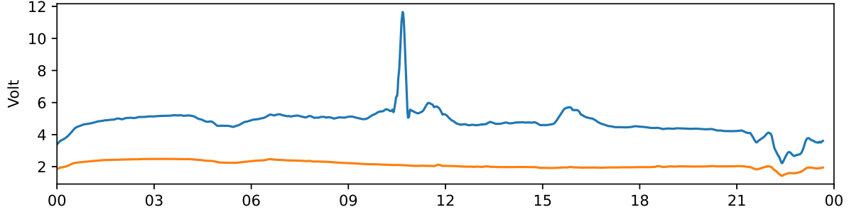
Tjautjas 30 MHz and 38 MHz riometer 2024-03-09 UTC
