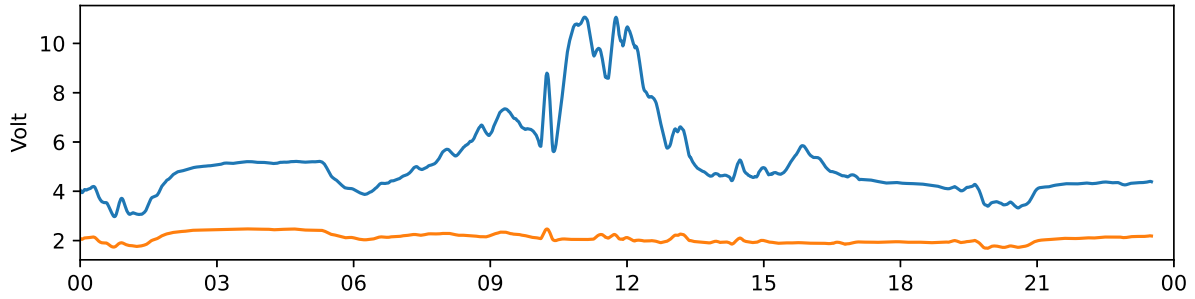
Tjautjas 30 MHz and 38 MHz riometer 2024-03-10 UTC
