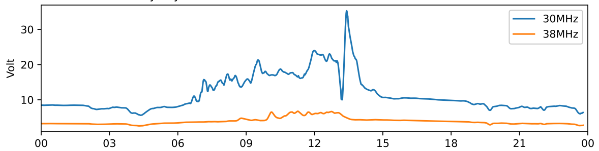
Tjautjas 30 MHz and 38 MHz riometer 2023-11-09 UTC
