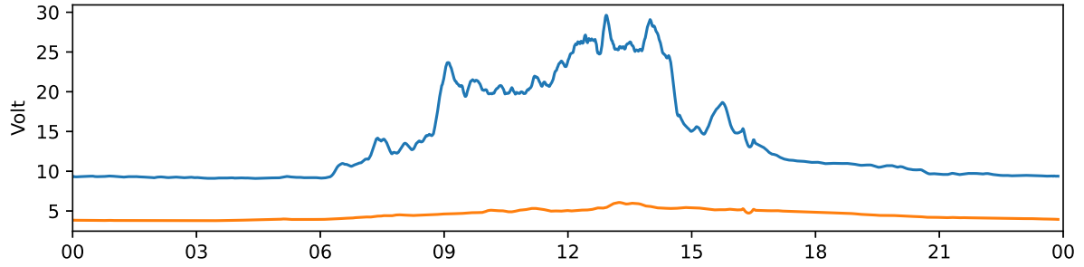
Tjautjas 30 MHz and 38 MHz riometer 2023-10-15 UTC
