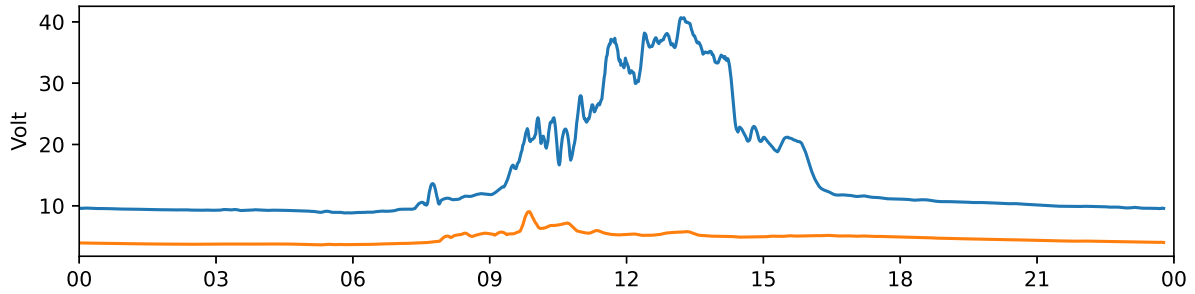
Tjautjas 30 MHz and 38 MHz riometer 2023-10-11 UTC
