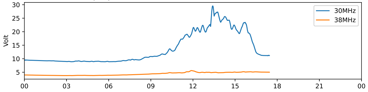
Tjautjas 30 MHz and 38 MHz riometer 2023-10-08 UTC
