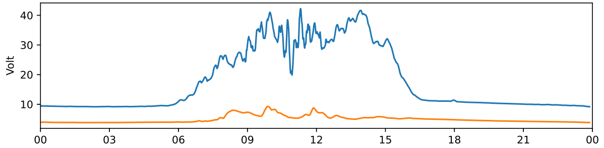
Tjautjas 30 MHz and 38 MHz riometer 2023-10-16 UTC
