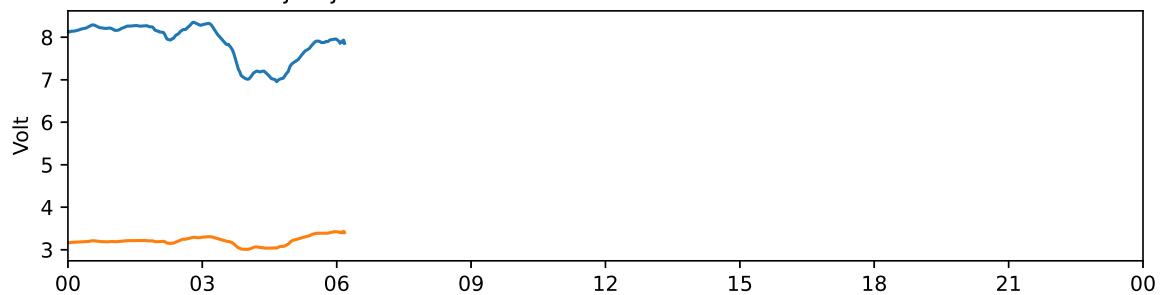
Tjautjas 30 MHz and 38 MHz riometer 2023-12-03 UTC
