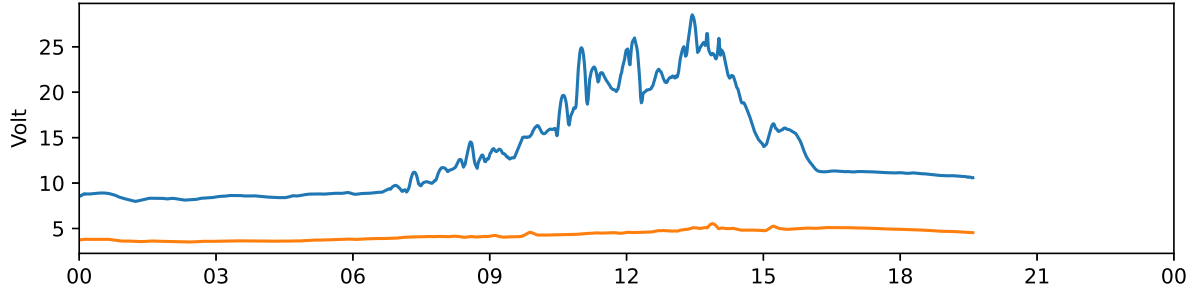
Tjautjas 30 MHz and 38 MHz riometer 2023-10-09 UTC
