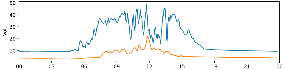
Tjautjas 30 MHz and 38 MHz riometer 2023-10-17 UTC
