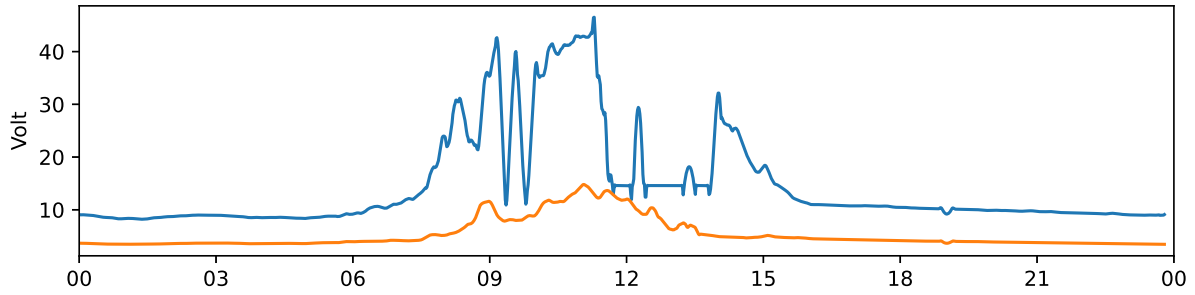
Tjautjas 30 MHz and 38 MHz riometer 2023-11-03 UTC
