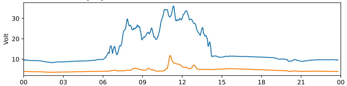
Tjautjas 30 MHz and 38 MHz riometer 2023-10-23 UTC
