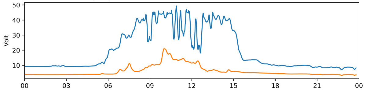
Tjautjas 30 MHz and 38 MHz riometer 2023-10-18 UTC
