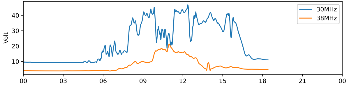
Tjautjas 30 MHz and 38 MHz riometer 2023-10-14 UTC
