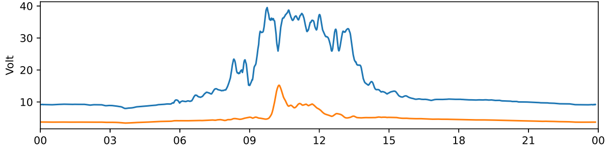
Tjautjas 30 MHz and 38 MHz riometer 2023-11-02 UTC
