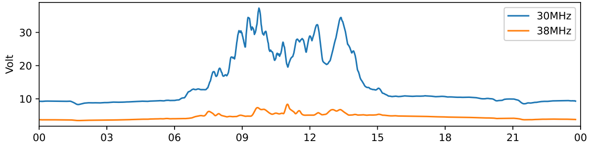
Tjautjas 30 MHz and 38 MHz riometer 2023-11-01 UTC
