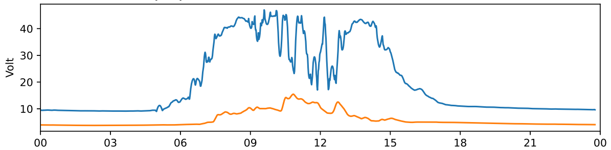
Tjautjas 30 MHz and 38 MHz riometer 2023-10-12 UTC
