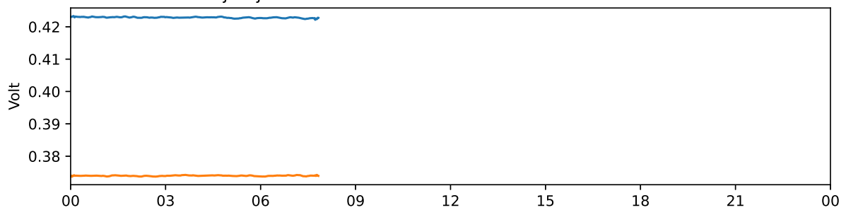
Tjautjas 30 MHz and 38 MHz riometer 2023-12-04 UTC
