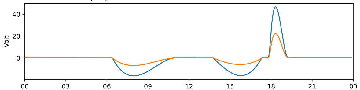
Tjautjas 30 MHz and 38 MHz riometer 2023-12-21 UTC
