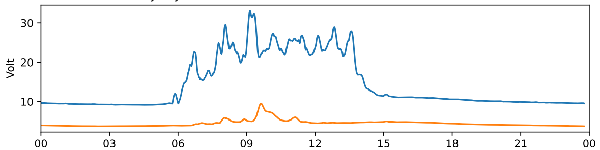
Tjautjas 30 MHz and 38 MHz riometer 2023-10-24 UTC
