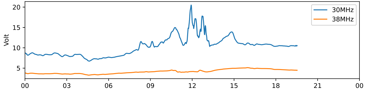
Tjautjas 30 MHz and 38 MHz riometer 2023-10-20 UTC
