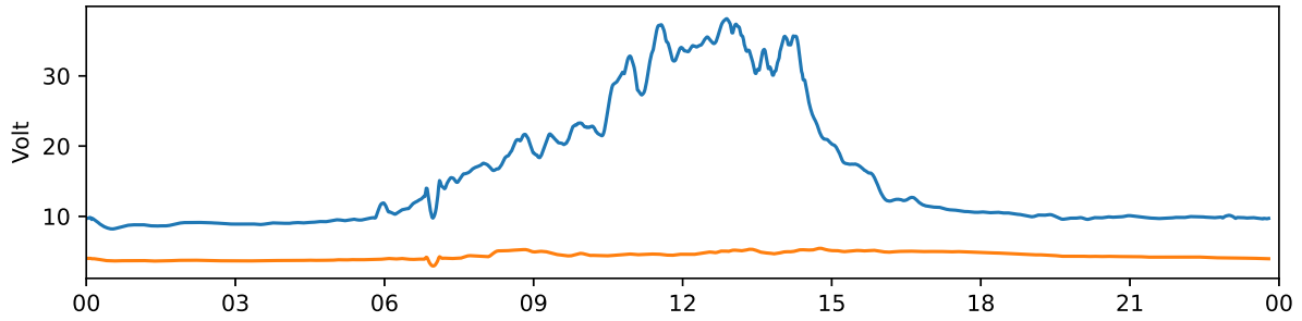
Tjautjas 30 MHz and 38 MHz riometer 2023-10-10 UTC
