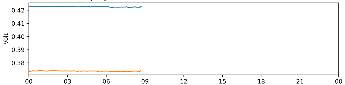
Tjautjas 30 MHz and 38 MHz riometer 2023-12-21 UTC
