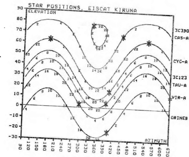
Figure A3. Star positions in Kiruna. Greenwich mean sidereal times at two-hour intervals are plotted.
