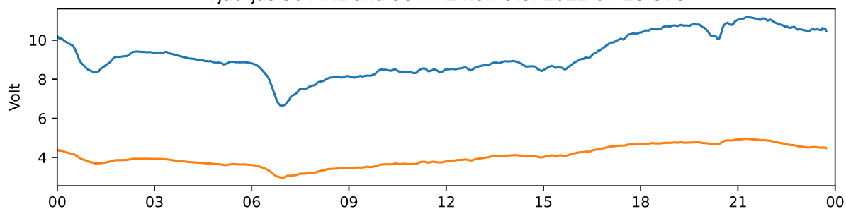
Tjautjas 30 MHz and 38 MHz riometer 2022-07-29 UTC
