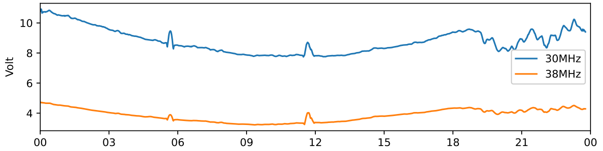
Tjautjas 30 MHz and 38 MHz riometer 2022-07-02 UTC
