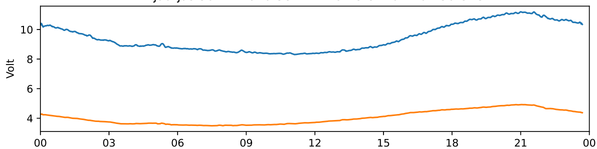
Tjautjas 30 MHz and 38 MHz riometer 2022-07-30 UTC
