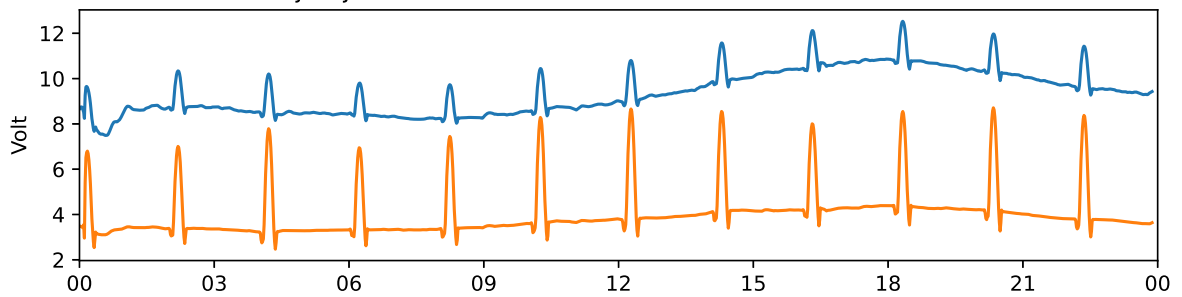
Tjautjas 30 MHz and 38 MHz riometer 2022-09-16 UTC
