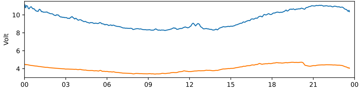
Tjautjas 30 MHz and 38 MHz riometer 2022-07-15 UTC
