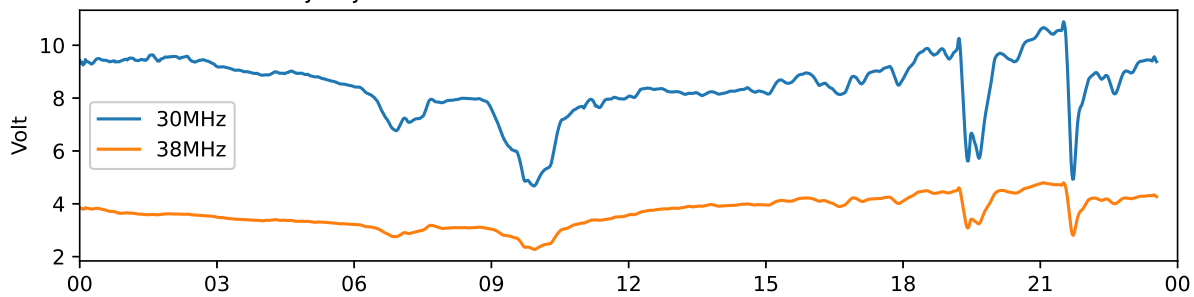
Tjautjas 30 MHz and 38 MHz riometer 2022-07-20 UTC
