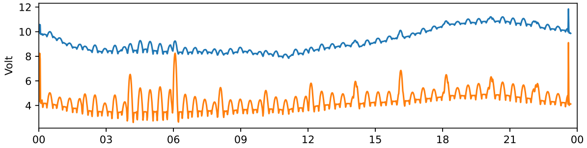
Tjautjas 30 MHz and 38 MHz riometer 2022-08-26 UTC
