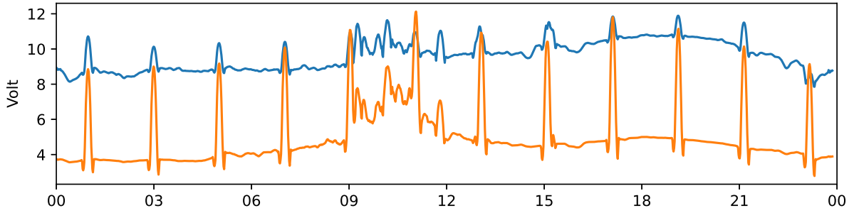
Tjautjas 30 MHz and 38 MHz riometer 2022-09-20 UTC
