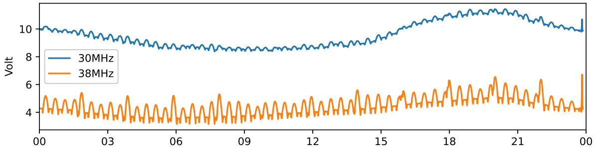
Tjautjas 30 MHz and 38 MHz riometer 2022-08-25 UTC
