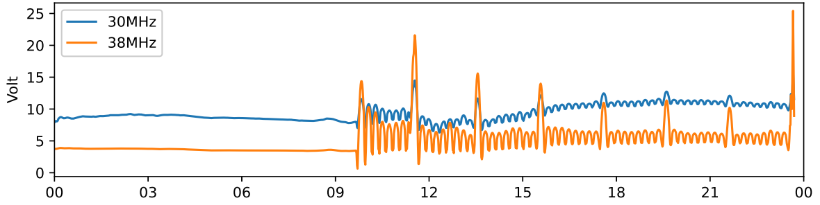
Tjautjas 30 MHz and 38 MHz riometer 2022-08-13 UTC
