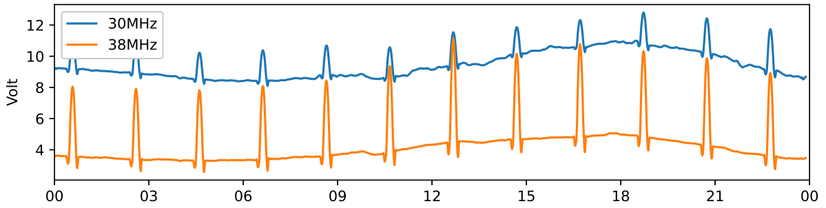
Tjautjas 30 MHz and 38 MHz riometer 2022-09-18 UTC
