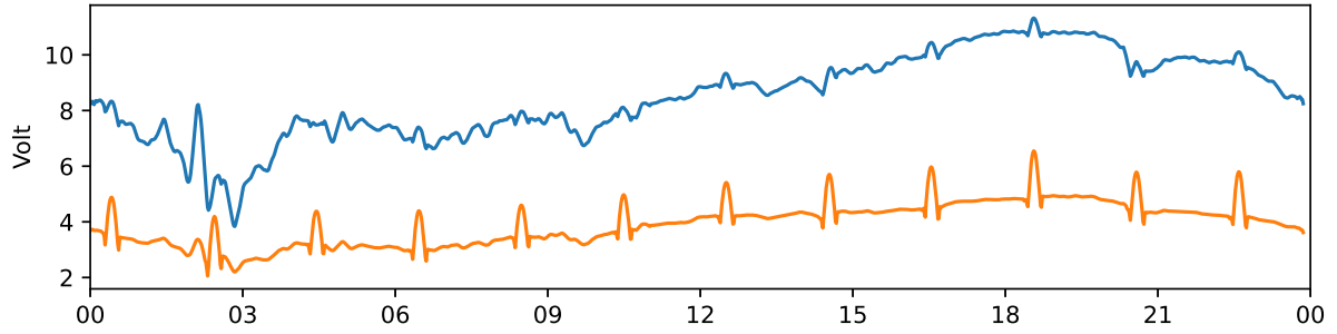
Tjautjas 30 MHz and 38 MHz riometer 2022-09-07 UTC
