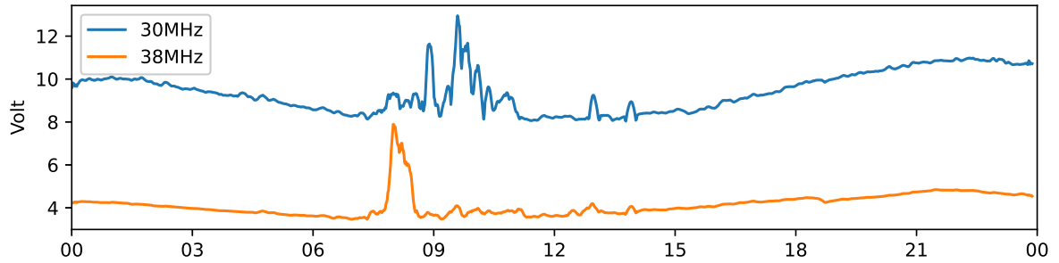
Tjautjas 30 MHz and 38 MHz riometer 2022-07-14 UTC
