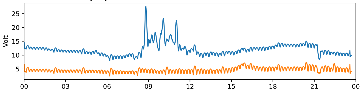
Tjautjas 30 MHz and 38 MHz riometer 2022-08-17 UTC
