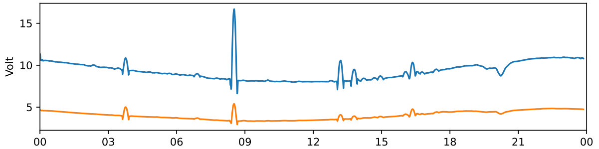
Tjautjas 30 MHz and 38 MHz riometer 2022-07-04 UTC
