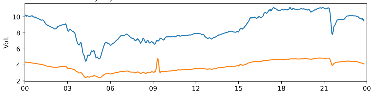
Tjautjas 30 MHz and 38 MHz riometer 2022-07-24 UTC
