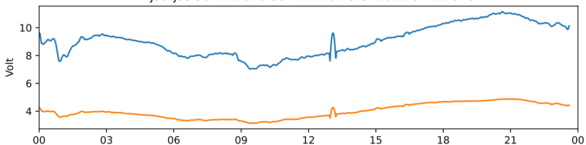
Tjautjas 30 MHz and 38 MHz riometer 2022-07-23 UTC
