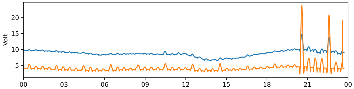
Tjautjas 30 MHz and 38 MHz riometer 2022-08-28 UTC
