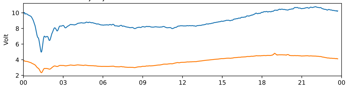
Tjautjas 30 MHz and 38 MHz riometer 2022-07-27 UTC
