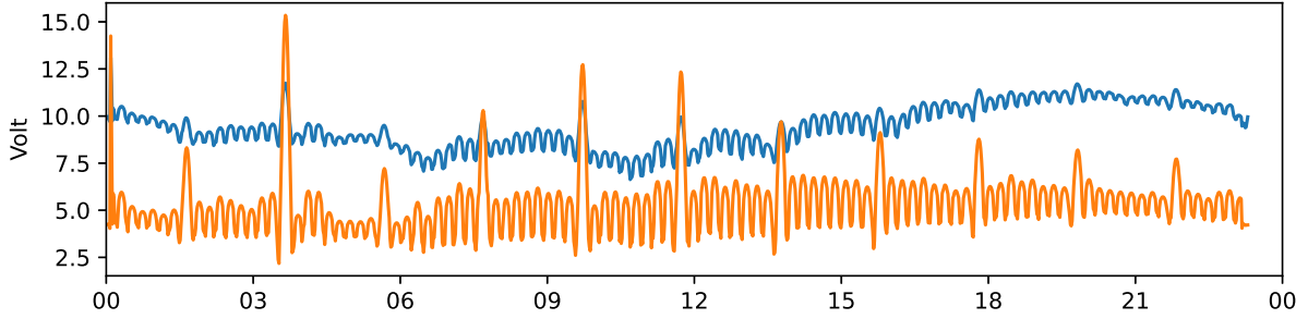
Tjautjas 30 MHz and 38 MHz riometer 2022-08-14 UTC
