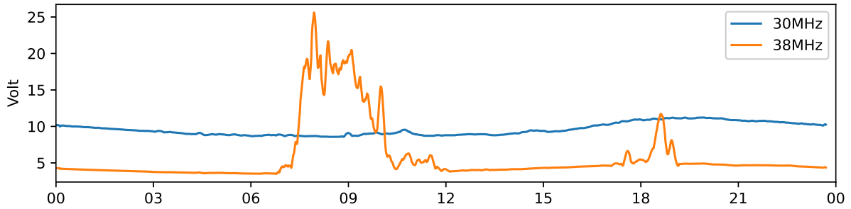
Tjautjas 30 MHz and 38 MHz riometer 2022-08-07 UTC
