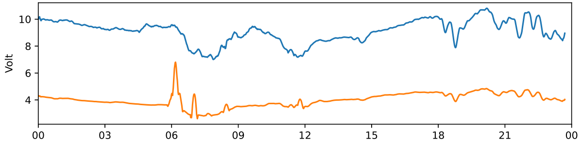
Tjautjas 30 MHz and 38 MHz riometer 2022-08-08 UTC
