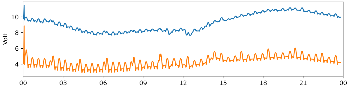
Tjautjas 30 MHz and 38 MHz riometer 2022-08-27 UTC
