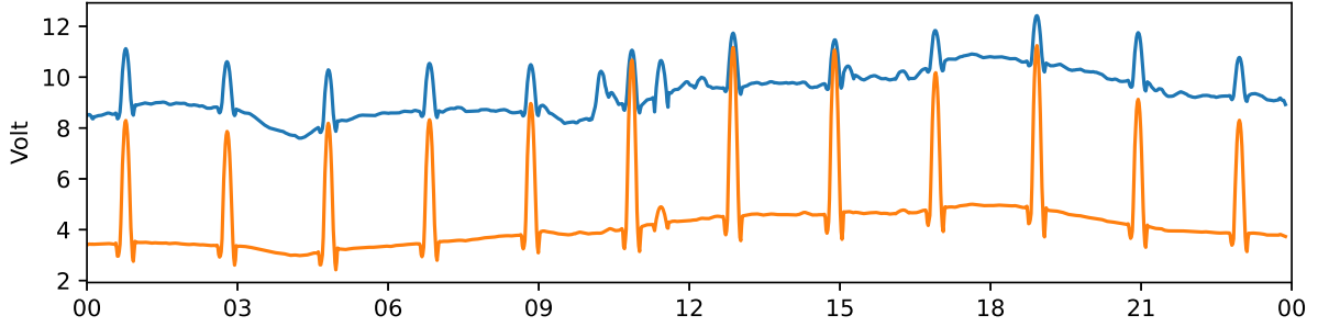
Tjautjas 30 MHz and 38 MHz riometer 2022-09-19 UTC
