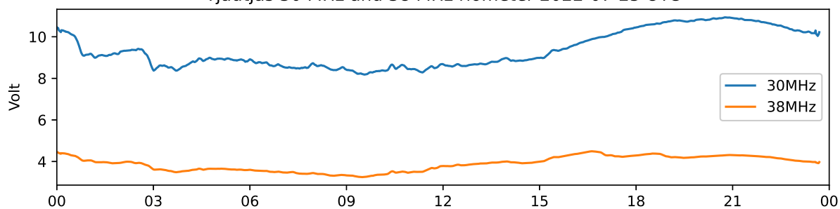
Tjautjas 30 MHz and 38 MHz riometer 2022-07-26 UTC
