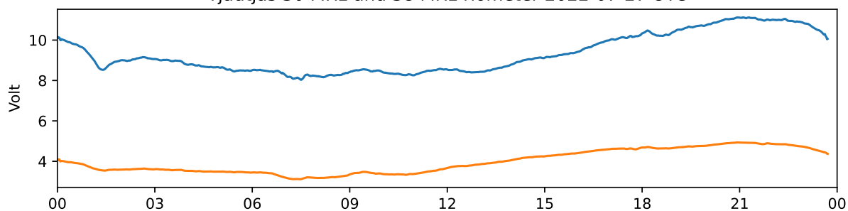
Tjautjas 30 MHz and 38 MHz riometer 2022-07-28 UTC
