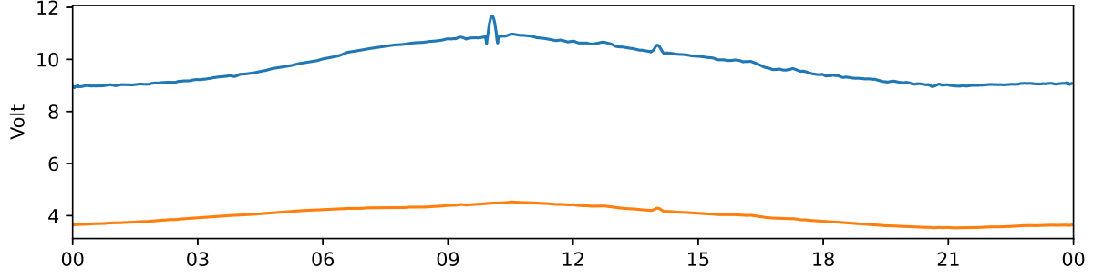
Kiruna 30 MHz and 38 MHz riometer 2021-12-31 UTC
