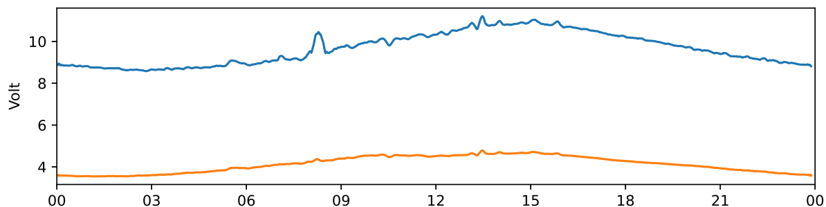
Kiruna 30 MHz and 38 MHz riometer 2021-10-29 UTC
