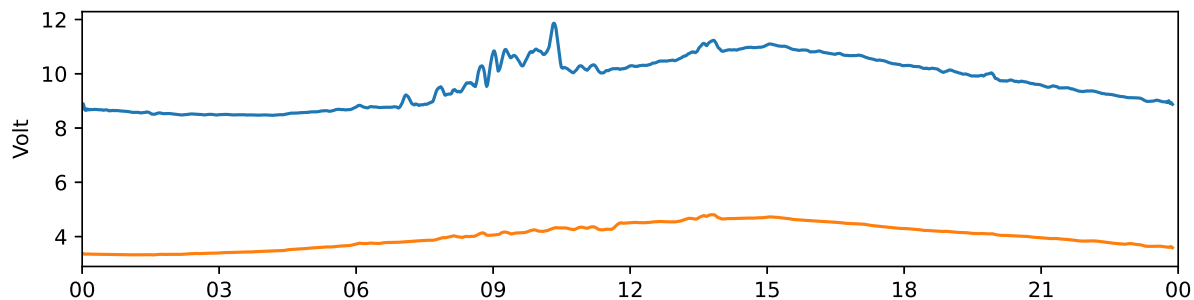
Kiruna 30 MHz and 38 MHz riometer 2021-10-28 UTC
