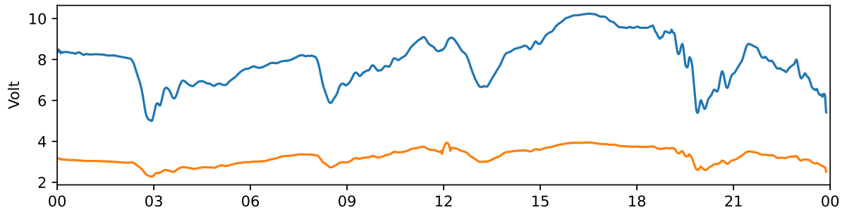
Kiruna 30 MHz and 38 MHz riometer 2021-10-12 UTC
