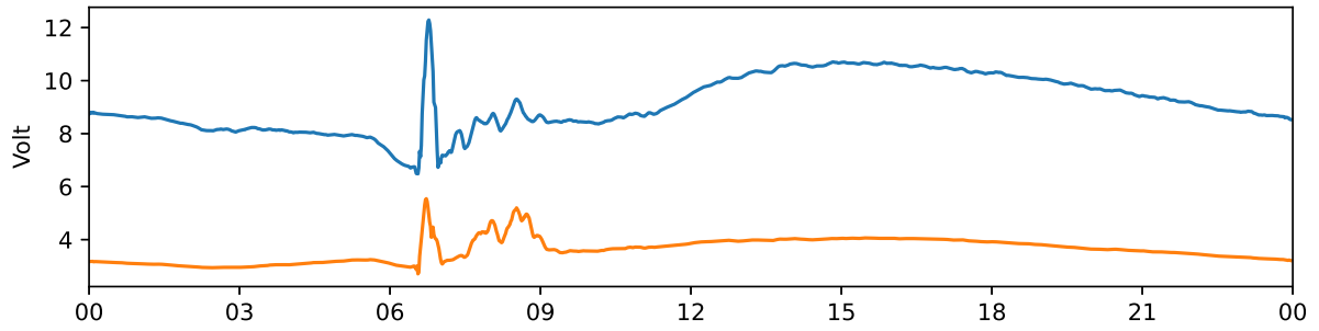
Kiruna 30 MHz and 38 MHz riometer 2021-10-10 UTC
