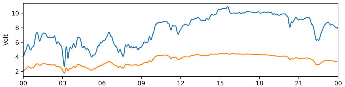
Kiruna 30 MHz and 38 MHz riometer 2021-10-12 UTC
