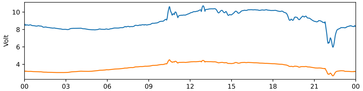
Kiruna 30 MHz and 38 MHz riometer 2021-10-11 UTC
