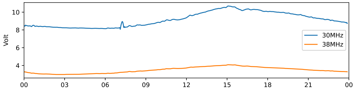
Kiruna 30 MHz and 38 MHz riometer 2021-10-08 UTC
