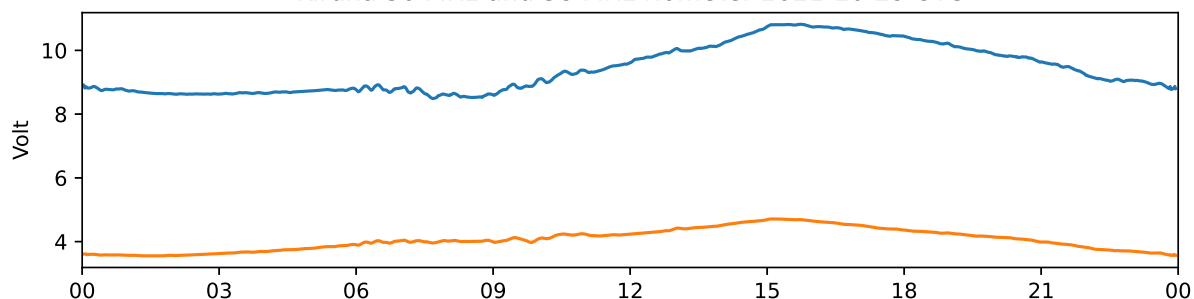
Kiruna 30 MHz and 38 MHz riometer 2021-10-30 UTC
