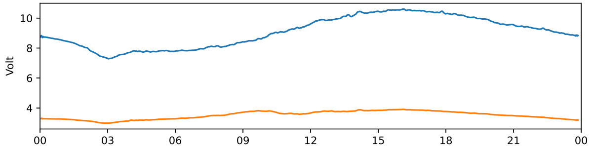
Kiruna 30 MHz and 38 MHz riometer 2021-10-09 UTC
