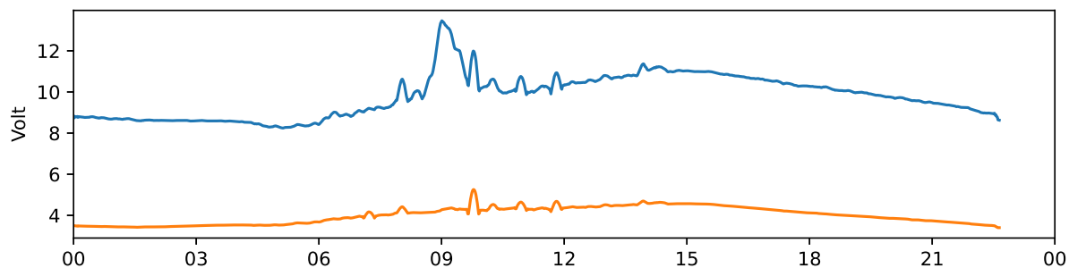
Kiruna 30 MHz and 38 MHz riometer 2021-10-27 UTC
