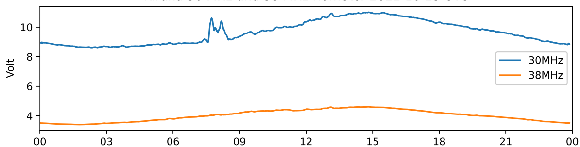
Kiruna 30 MHz and 38 MHz riometer 2021-10-26 UTC
