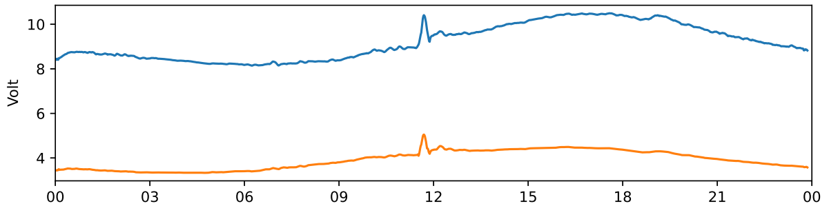
Kiruna 30 MHz and 38 MHz riometer 2021-09-27 UTC
