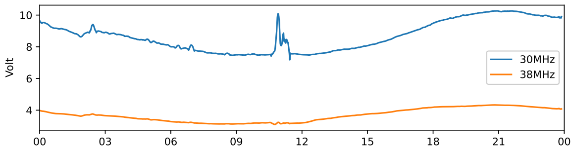
Kiruna 30 MHz and 38 MHz riometer 2021-07-14 UTC
