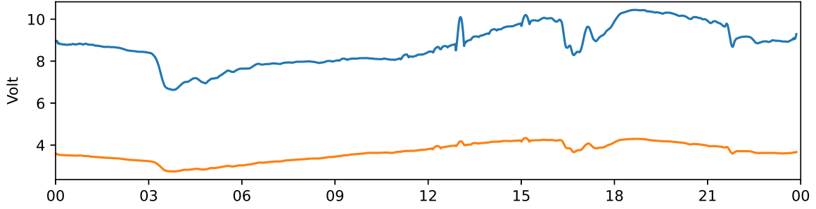
Kiruna 30 MHz and 38 MHz riometer 2021-09-07 UTC
