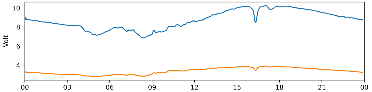
Kiruna 30 MHz and 38 MHz riometer 2021-09-25 UTC
