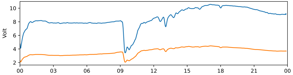
Kiruna 30 MHz and 38 MHz riometer 2021-09-09 UTC
