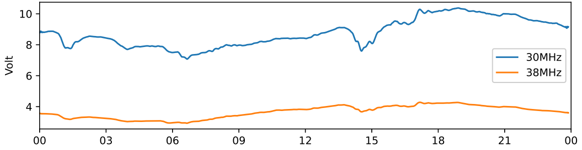
Kiruna 30 MHz and 38 MHz riometer 2021-09-06 UTC
