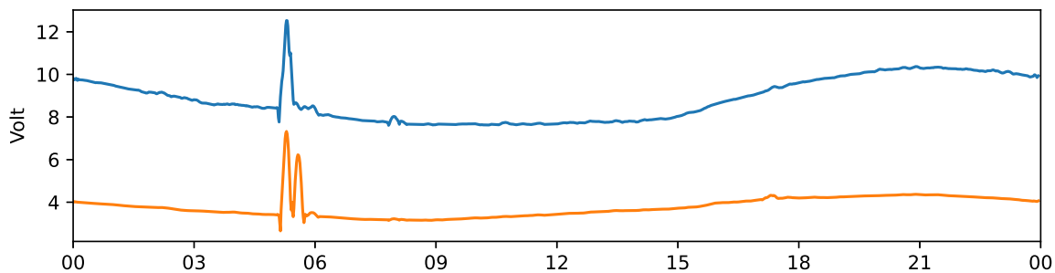
Kiruna 30 MHz and 38 MHz riometer 2021-07-18 UTC
