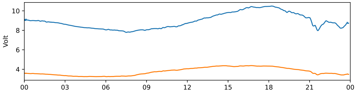
Kiruna 30 MHz and 38 MHz riometer 2021-09-10 UTC
