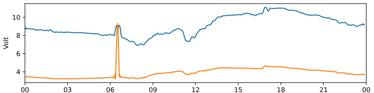
Kiruna 30 MHz and 38 MHz riometer 2021-09-28 UTC
