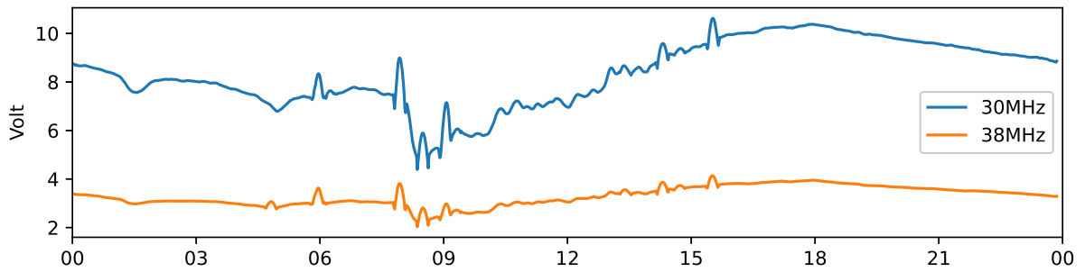
Kiruna 30 MHz and 38 MHz riometer 2021-09-24 UTC
