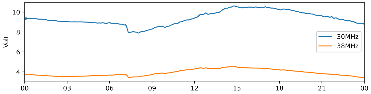
Kiruna 30 MHz and 38 MHz riometer 2021-09-30 UTC
