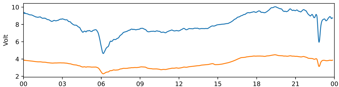
Kiruna 30 MHz and 38 MHz riometer 2021-07-16 UTC
