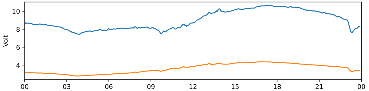
Kiruna 30 MHz and 38 MHz riometer 2021-09-26 UTC
