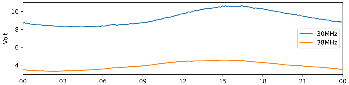
Kiruna 30 MHz and 38 MHz riometer 2020-10-14 UTC
