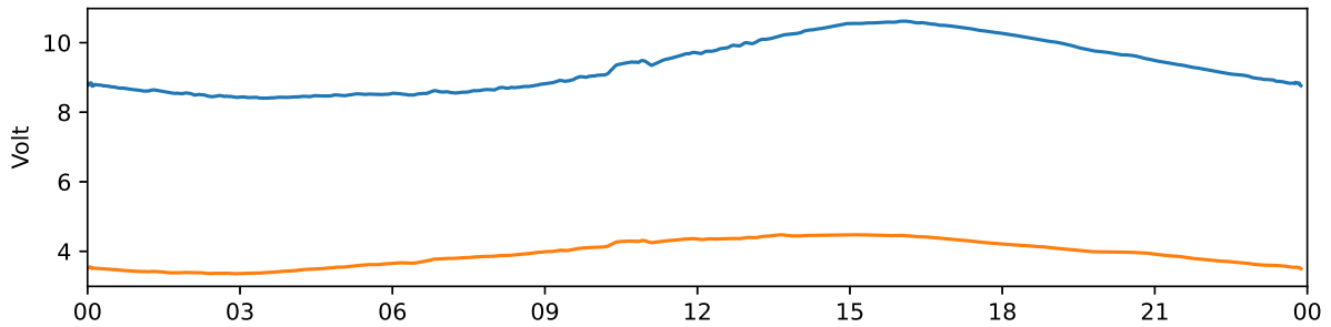
Kiruna 30 MHz and 38 MHz riometer 2020-10-15 UTC
