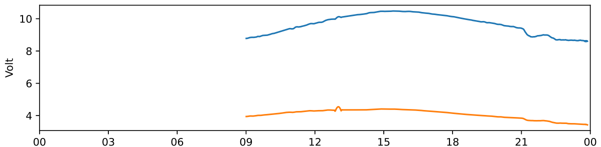
Kiruna 30 MHz and 38 MHz riometer 2020-10-17 UTC
