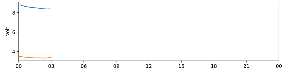
Kiruna 30 MHz and 38 MHz riometer 2020-10-16 UTC
