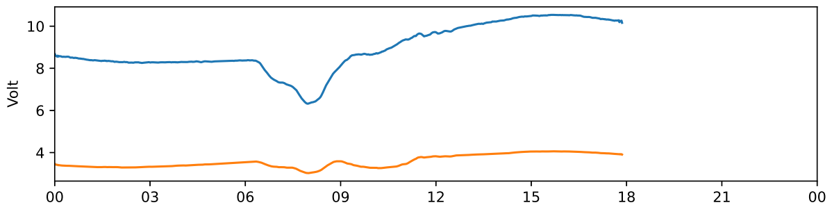
Kiruna 30 MHz and 38 MHz riometer 2020-10-19 UTC
