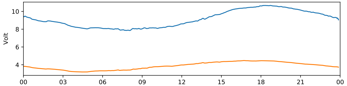
Kiruna 30 MHz and 38 MHz riometer 2020-09-04 UTC
