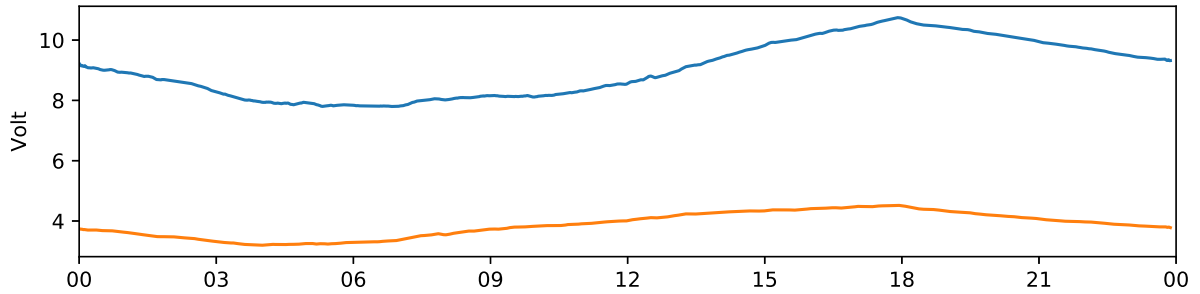
Kiruna 30 MHz and 38 MHz riometer 2020-09-10 UTC
