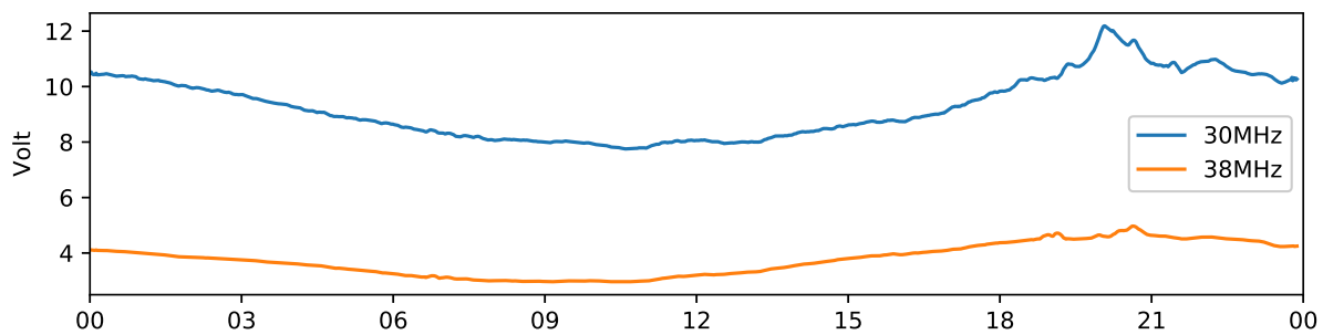
Kiruna 30 MHz and 38 MHz riometer 2020-07-02 UTC
