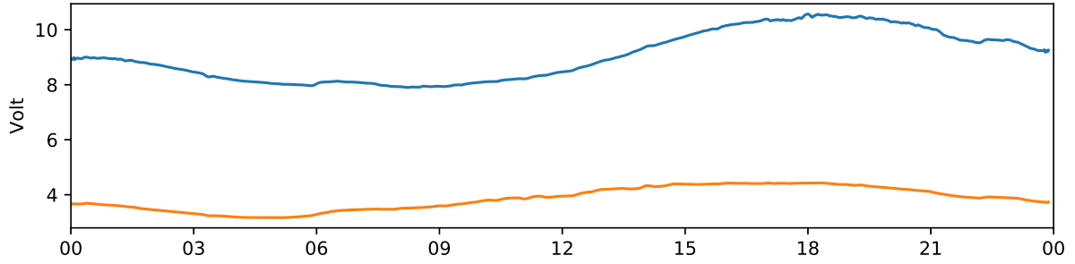
Kiruna 30 MHz and 38 MHz riometer 2020-09-08 UTC
