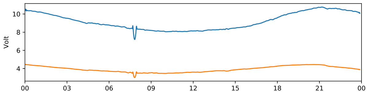
Kiruna 30 MHz and 38 MHz riometer 2020-07-04 UTC
