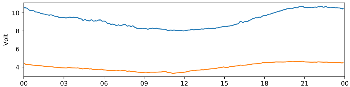
Kiruna 30 MHz and 38 MHz riometer 2020-07-03 UTC
