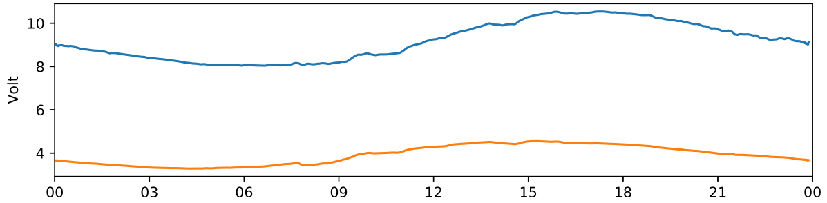
Kiruna 30 MHz and 38 MHz riometer 2020-09-21 UTC
