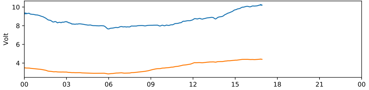
Kiruna 30 MHz and 38 MHz riometer 2020-09-07 UTC
