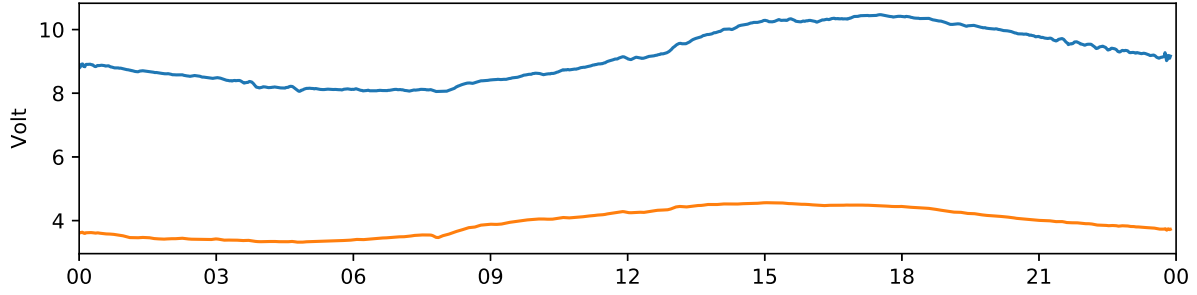
Kiruna 30 MHz and 38 MHz riometer 2020-09-19 UTC
