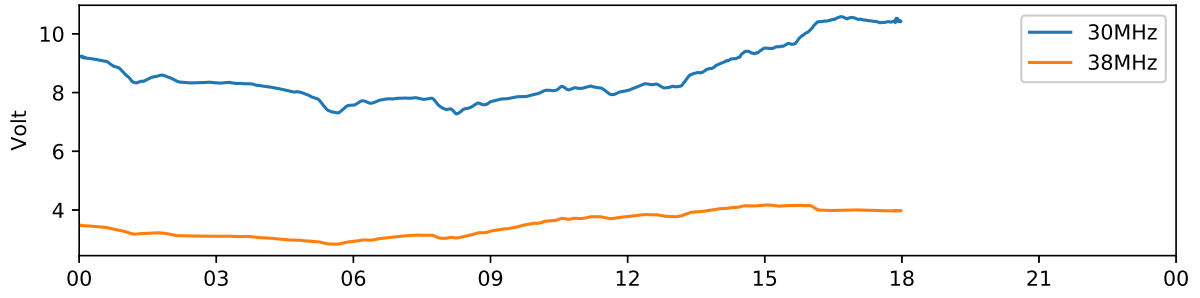
Kiruna 30 MHz and 38 MHz riometer 2020-09-06 UTC
