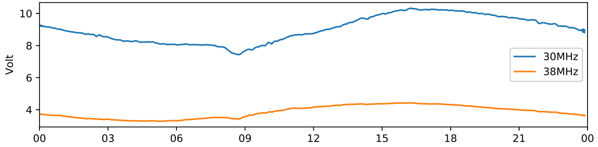
Kiruna 30 MHz and 38 MHz riometer 2020-09-18 UTC
