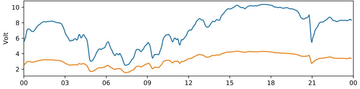
Kiruna 30 MHz and 38 MHz riometer 2020-09-30 UTC
