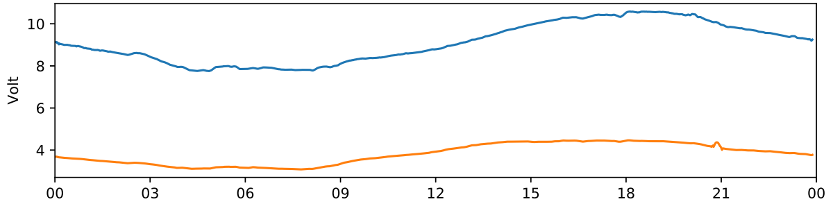
Kiruna 30 MHz and 38 MHz riometer 2020-09-09 UTC
