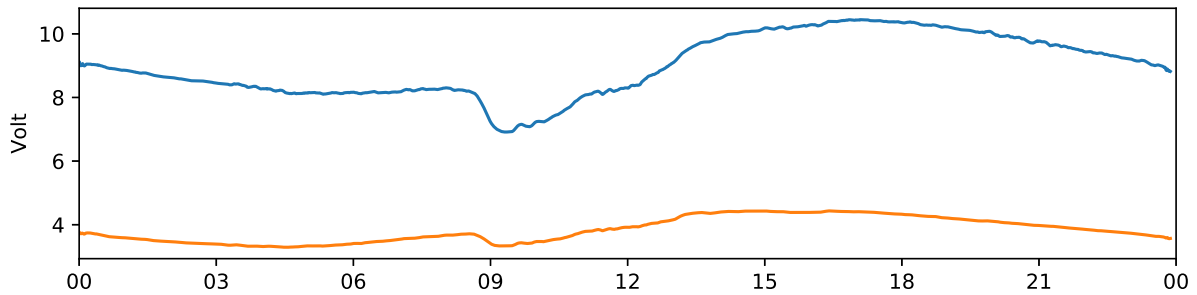
Kiruna 30 MHz and 38 MHz riometer 2020-09-22 UTC
