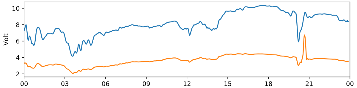
Kiruna 30 MHz and 38 MHz riometer 2020-09-01 UTC
