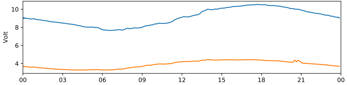
Kiruna 30 MHz and 38 MHz riometer 2020-09-20 UTC
