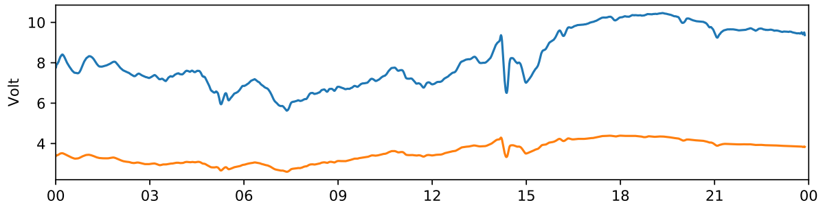
Kiruna 30 MHz and 38 MHz riometer 2020-09-03 UTC
