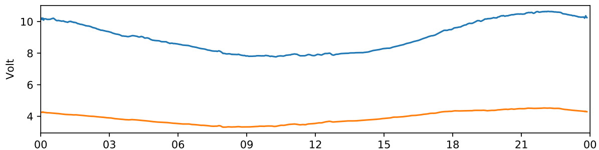
Kiruna 30 MHz and 38 MHz riometer 2020-07-06 UTC
