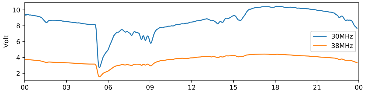
Kiruna 30 MHz and 38 MHz riometer 2020-08-31 UTC
