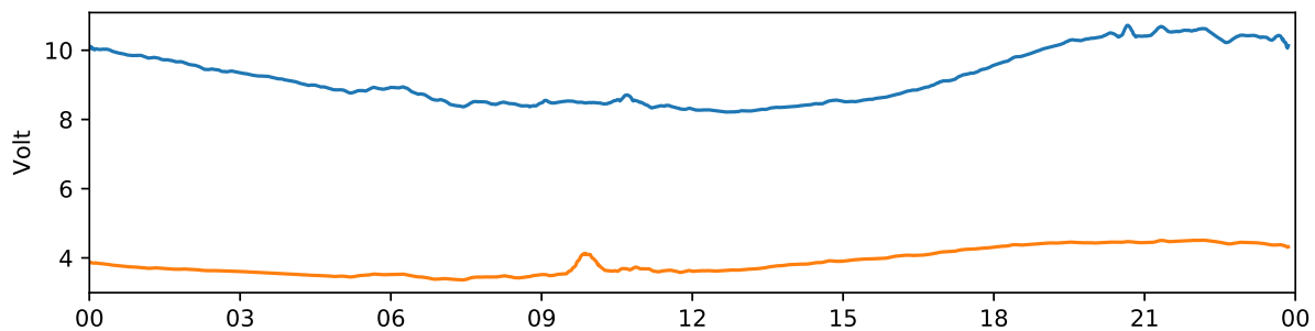
Kiruna 30 MHz and 38 MHz riometer 2020-07-05 UTC
