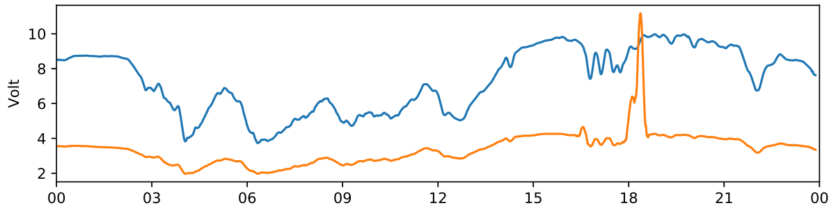
Kiruna 30 MHz and 38 MHz riometer 2020-09-02 UTC
