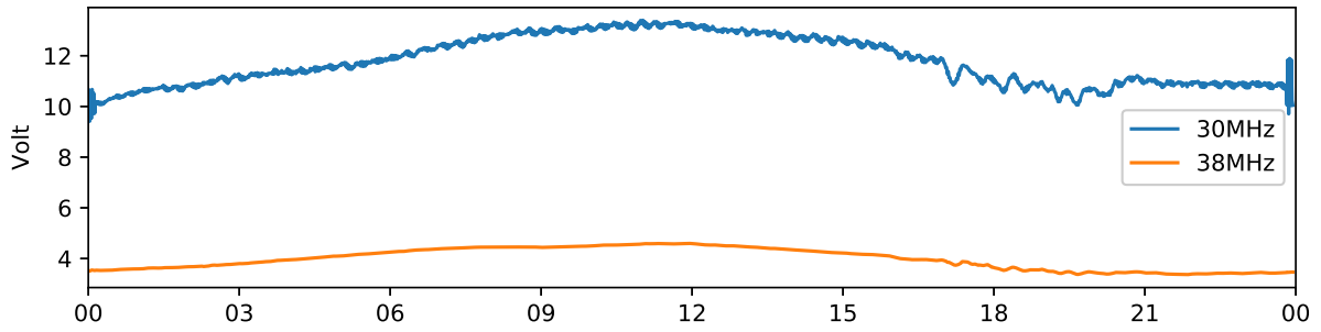
Kiruna 30 MHz and 38 MHz riometer 2019-12-19 UTC
