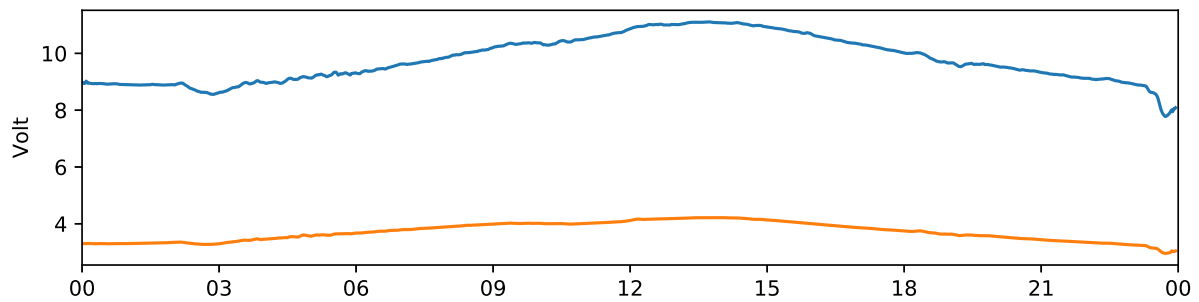
Kiruna 30 MHz and 38 MHz riometer 2019-11-17 UTC
