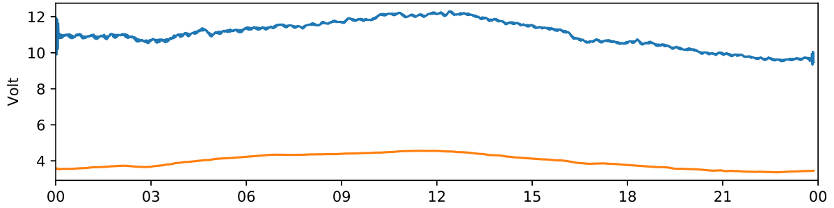
Kiruna 30 MHz and 38 MHz riometer 2019-12-21 UTC
