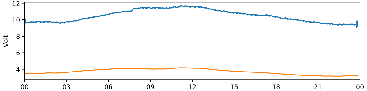
Kiruna 30 MHz and 38 MHz riometer 2019-12-22 UTC
