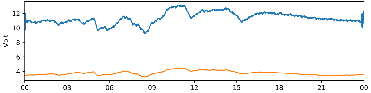
Kiruna 30 MHz and 38 MHz riometer 2019-12-20 UTC
