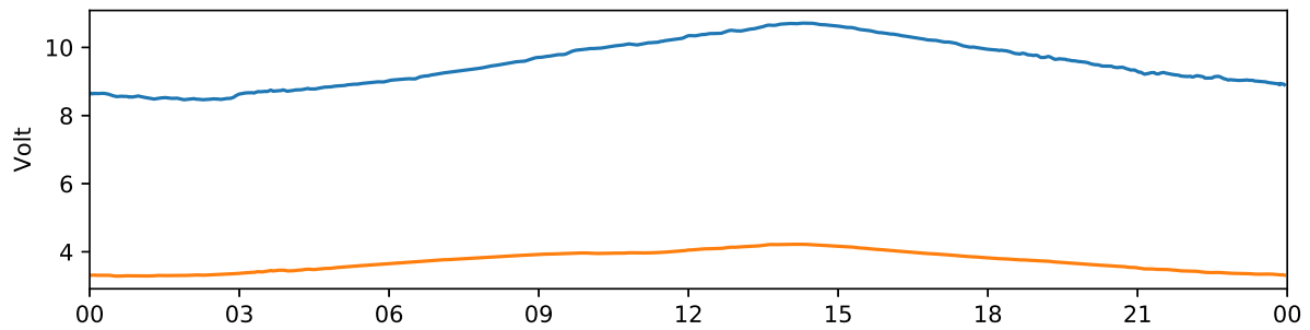
Kiruna 30 MHz and 38 MHz riometer 2019-11-15 UTC
