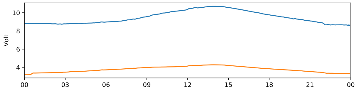
Kiruna 30 MHz and 38 MHz riometer 2019-11-14 UTC
